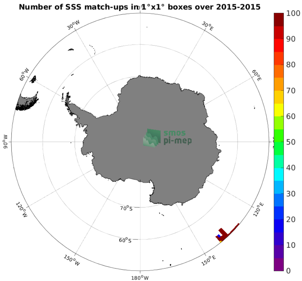
Figure 4: Number of SSS match-ups between TSG (GOSUD-Research-vessel) SSS and the Aquarius SSS L3 OR v5 - 7-Day running - Rain mask (NASA-GSFC) SSS product for the Southern Ocean Pi-MEP region over 1^\circ \times 1^\circ boxes and for the full satellite product period.
