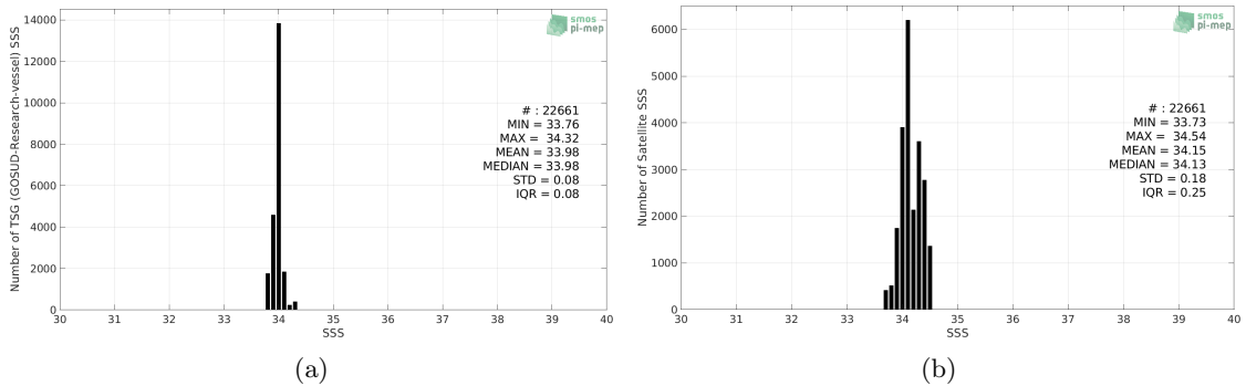
Figure 2: Histograms of SSS from TSG (GOSUD-Research-vessel) (a) and Aquarius SSS L3 OR v5 - 7-Day running - Rain mask (NASA-GSFC) (b) considering all match-up pairs per bins of 0.1 over the Southern Ocean Pi-MEP region and for the full satellite product period.
