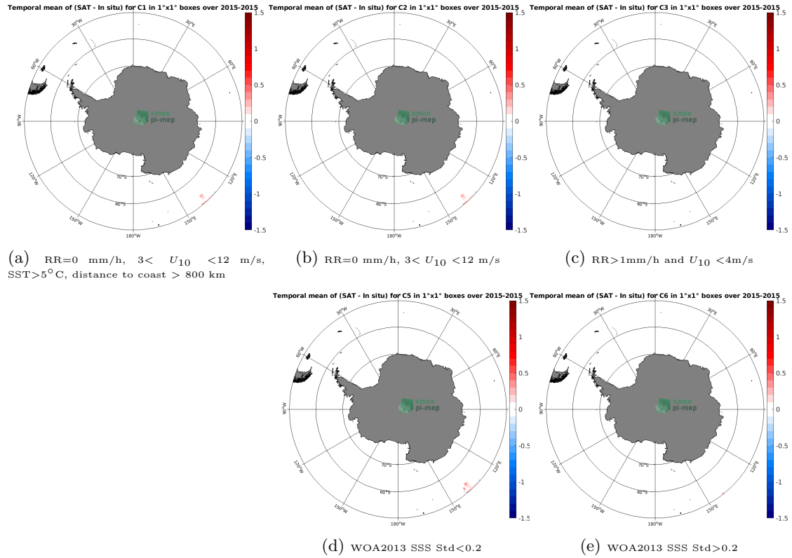
Figure 12: Temporal mean gridded over spatial boxes of size 1^\circ \times 1^\circ of \Delta\text{SSS} (Aquarius SSS L3 OR v5 - 7-Day running - Rain mask (NASA-GSFC) - TSG (GOSUD-Research-vessel)) for 5 different subdatasets corresponding to: RR=0 mm/h, 3 < U_{10} < 12 m/s, SST > 5^\circ\text{C} , distance to coast > 800 km (a), RR=0 mm/h, 3 < U_{10} < 12 m/s (b), RR > 1 mm/h and U_{10} < 4 m/s (c), WOA2013 SSS Std < 0.2 (d), WOA2013 SSS Std > 0.2 (e).
