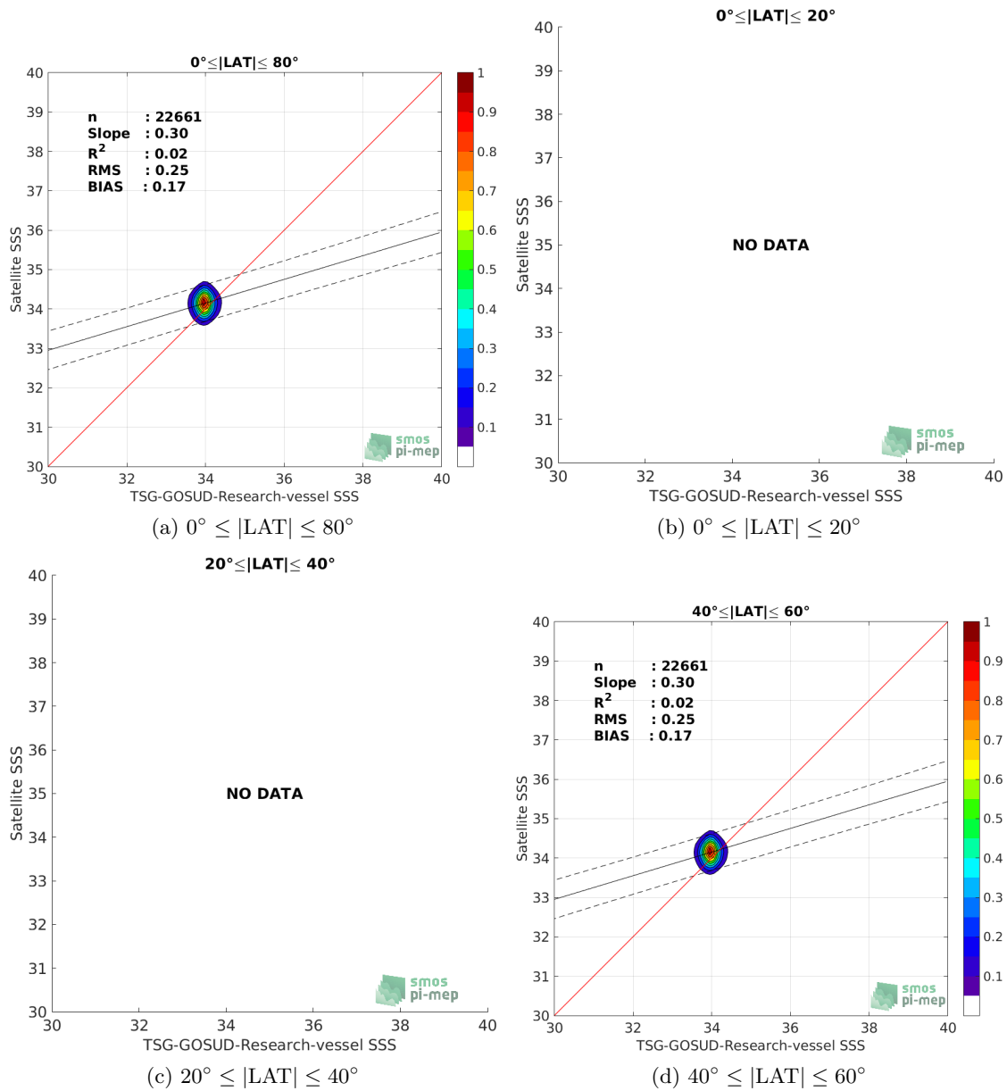
Figure 9: Contour maps of the concentration of Aquarius-L3-OR-V5-7DAY-RUNNING-RAIN-MASK-1DEG SSS (y-axis) versus TSG-GOSUD-Research-vessel SSS (x-axis) at match-up pairs for different latitude bands. For each plot, the red line shows x=y . The black thin and dashed lines indicate a linear fit through the data cloud and the \pm 95\% confidence levels, respectively. The number match-up pairs n , the slope and R^2 coefficient of the linear fit, the root mean square (RMS) and the mean bias between satellite and in situ data are indicated for each latitude band in each plots.
