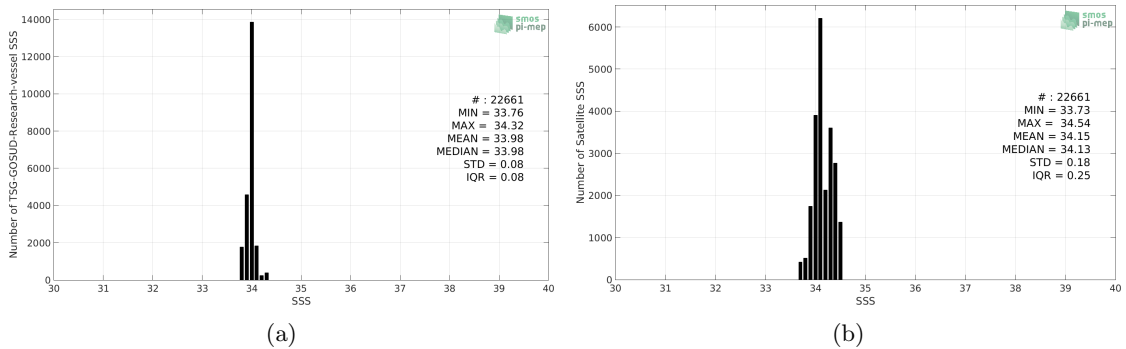
Figure 2: Histograms of SSS from TSG-GOSUD-Research-vessel (a) and Aquarius-L3-OR-V5-7DAY-RUNNING-RAIN-MASK-1DEG (b) considering all match-up pairs per bins of 0.1 over the Southern Ocean Pi-MEP region and for the full satellite product period.
