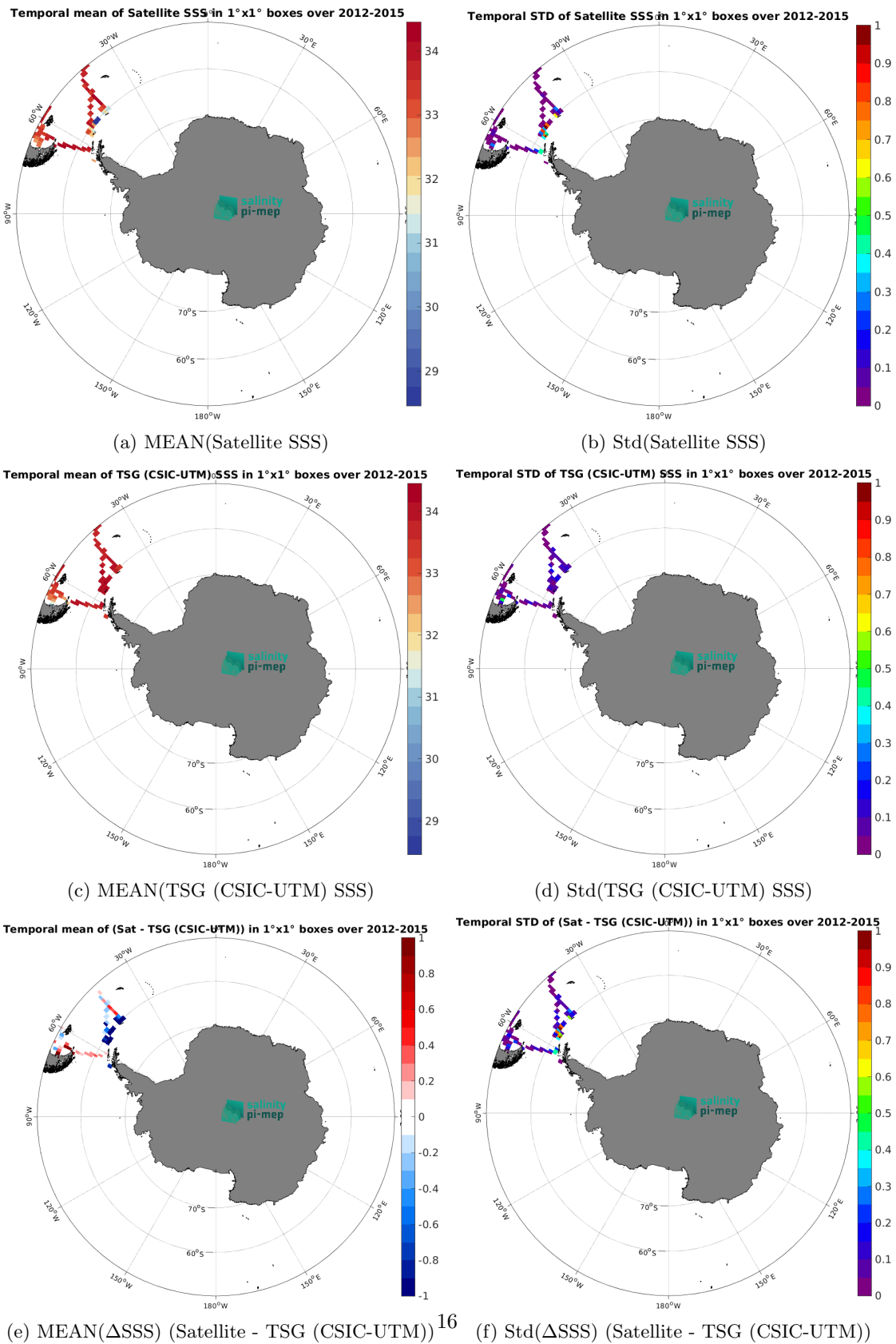
Figure 7: Temporal mean (left) and Std (right) of SSS from Aquarius SSS L3 OR v5 - 7-Day running - Rain mask (NASA-GSFC) (top), TSG (CSIC-UTM) (middle), and of \Delta SSS (Satellite - TSG (CSIC-UTM)). Only match-up pairs are used to generate these maps.
