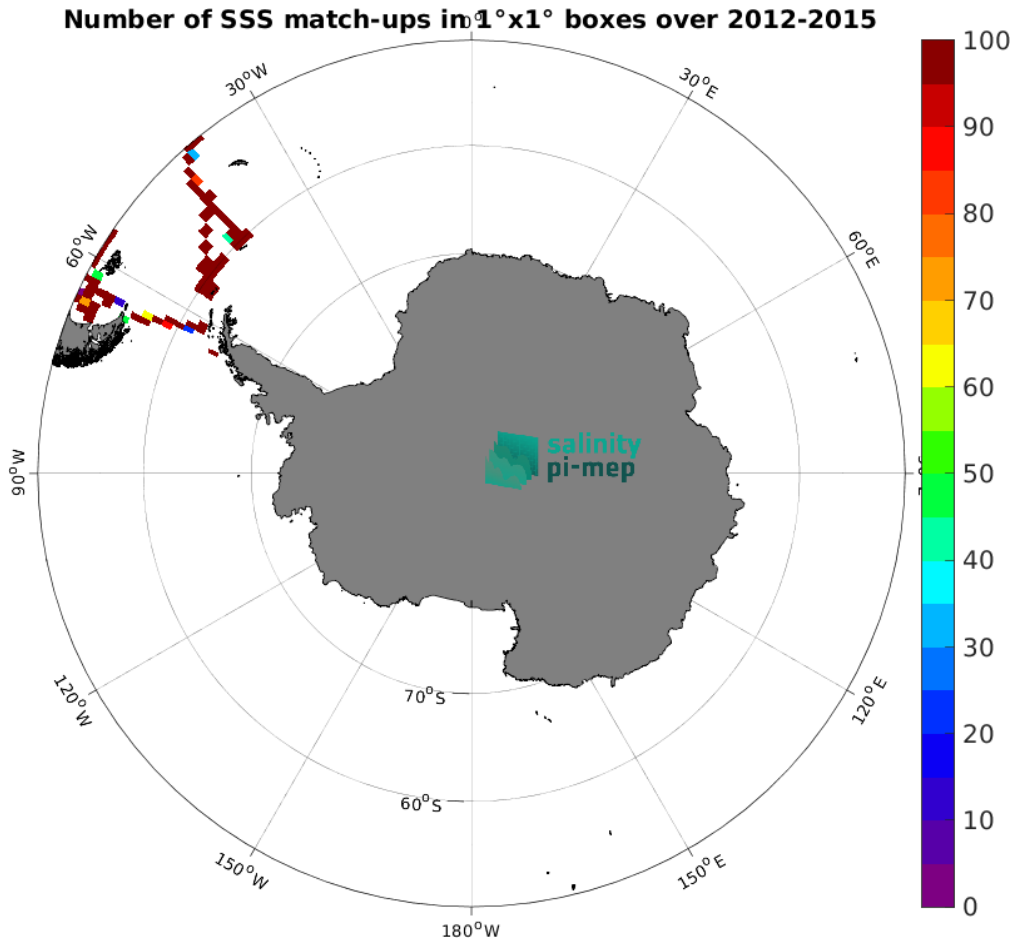
Figure 5: Number of SSS match-ups between TSG (CSIC-UTM) SSS and the Aquarius SSS L3 OR v5 - 7-Day running - Rain mask (NASA-GSFC) SSS product for the Southern Ocean Pi-MEP region over 1^\circ \times 1^\circ boxes and for the full satellite product period.
