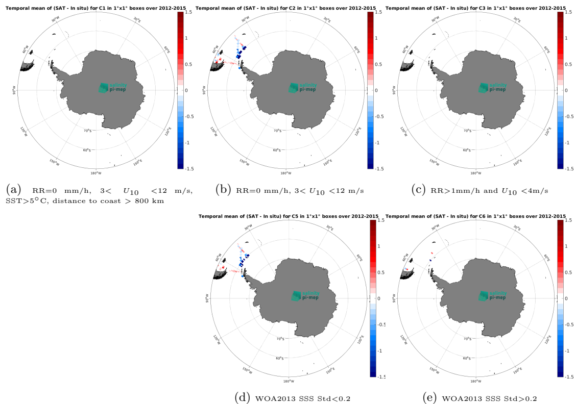
Figure 14: Temporal mean gridded over spatial boxes of size 1^\circ \times 1^\circ of \Delta SSS (Aquarius SSS L3 OR v5 - 7-Day running - Rain mask (NASA-GSFC) - TSG (CSIC-UTM)) for 5 different subdatasets corresponding to:RR=0 mm/h, 3 < U_{10} < 12 m/s, SST >5^\circ\text{C} , distance to coast > 800 km (a), RR=0 mm/h, 3 < U_{10} < 12 m/s (b), RR >1 mm/h and U_{10} < 4 m/s (c), WOA2013 SSS Std <0.2 (d), WOA2013 SSS Std >0.2 (e).
