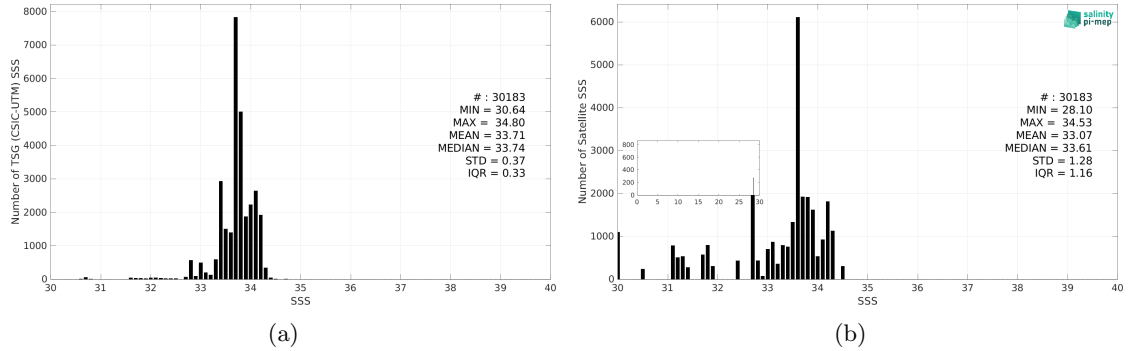
Figure 3: Histograms of SSS from TSG (CSIC-UTM) (a) and Aquarius SSS L3 OR v5 - 7-Day running - Rain mask (NASA-GSFC) (b) considering all match-up pairs per bins of 0.1 over the Southern Ocean Pi-MEP region and for the full satellite product period.
