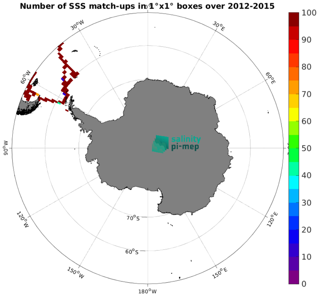
Figure 4: Number of SSS match-ups between TSG (CSIC-UTM) SSS and the Aquarius SSS L3 OR v5 - 7-Day running - Rain mask (NASA-GSFC) SSS product for the Southern Ocean Pi-MEP region over 1^\circ \times 1^\circ boxes and for the full satellite product period.
