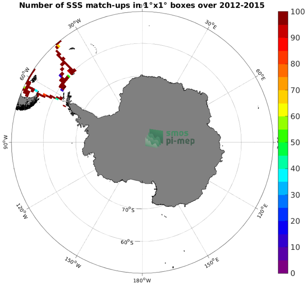
Figure 4: Number of SSS match-ups between TSG (CSIC-UTM) SSS and the Aquarius SSS L3 OR v5 - 7-Day running - Rain mask (NASA-GSFC) SSS product for the Southern Ocean Pi-MEP region over 1^\circ \times 1^\circ boxes and for the full satellite product period.
