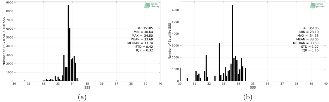
Figure 2: Histograms of SSS from TSG (CSIC-UTM) (a) and Aquarius SSS L3 OR v5 - 7-Day running - Rain mask (NASA-GSFC) (b) considering all match-up pairs per bins of 0.1 over the Southern Ocean Pi-MEP region and for the full satellite product period.
