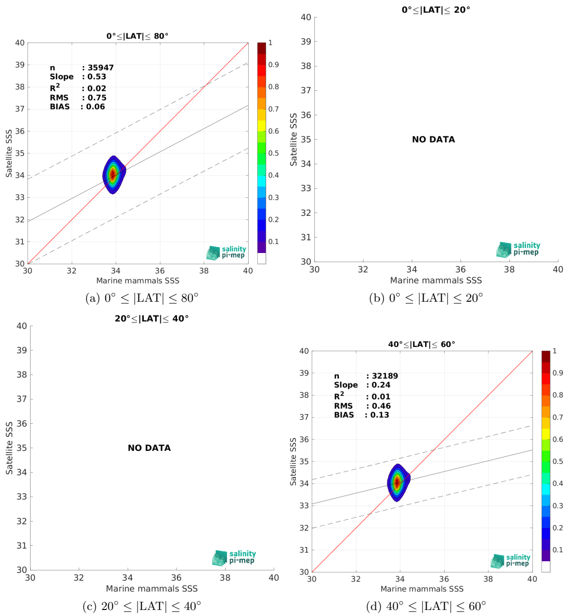
Figure 10: Contour maps of the concentration of Aquarius SSS L3 OR v5 - 7-Day running - Rain mask (NASA-GSFC) SSS (y-axis) versus Marine mammals SSS (x-axis) at match-up pairs for different latitude bands. For each plot, the red line shows x=y . The black thin and dashed lines indicate a linear fit through the data cloud and the \pm 95\% confidence levels, respectively. The number match-up pairs n , the slope and R^2 coefficient of the linear fit, the root mean square (RMS) and the mean bias between satellite and in situ data are indicated for each latitude band in each plots.
