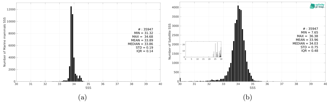
Figure 3: Histograms of SSS from Marine mammals (a) and Aquarius SSS L3 OR v5 - 7-Day running - Rain mask (NASA-GSFC) (b) considering all match-up pairs per bins of 0.1 over the Southern Ocean Pi-MEP region and for the full satellite product period.
