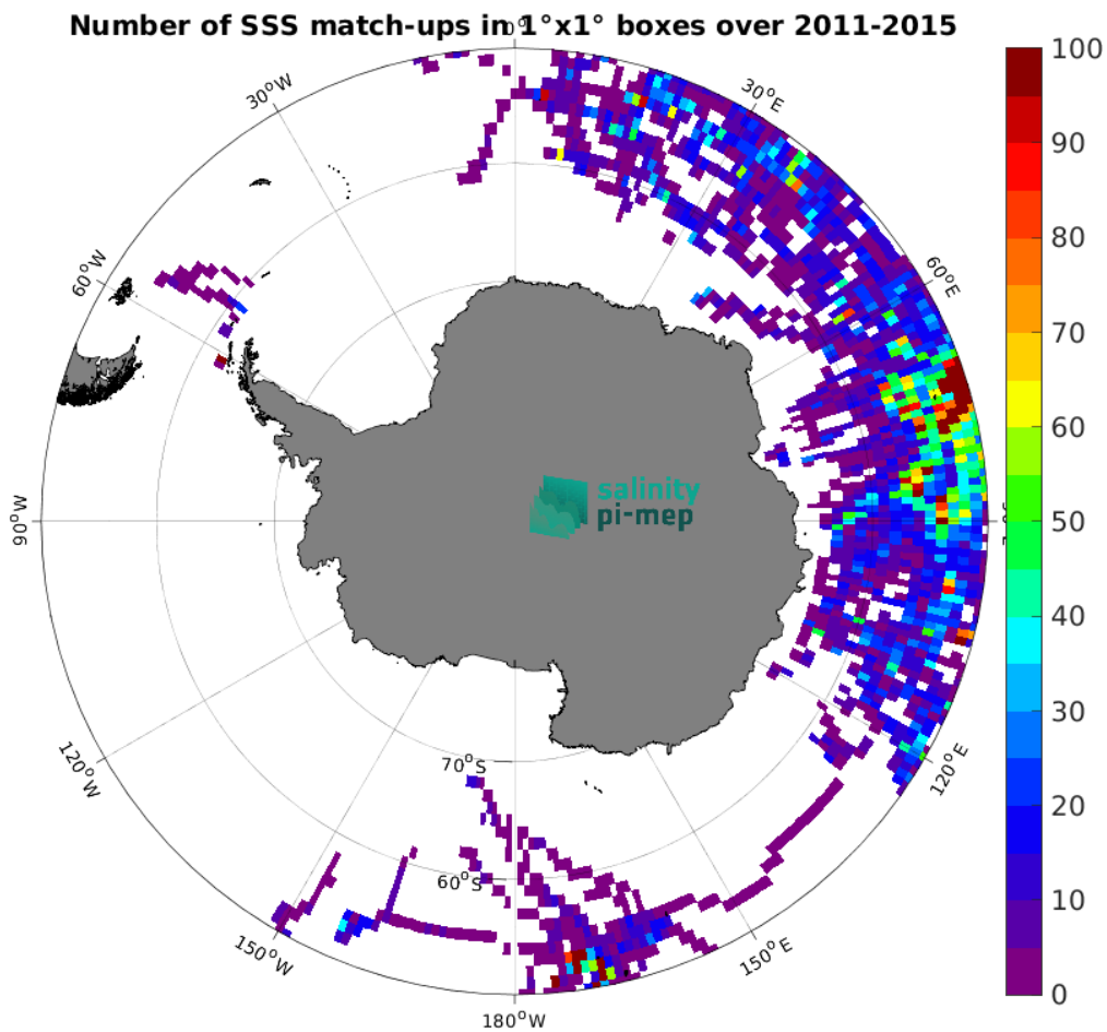
Figure 5: Number of SSS match-ups between Marine mammals SSS and the Aquarius SSS L3 OR v5 - 7-Day running - Rain mask (NASA-GSFC) SSS product for the Southern Ocean Pi-MEP region over 1^\circ \times 1^\circ boxes and for the full satellite product period.
