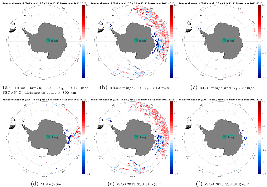
Figure 14: Temporal mean gridded over spatial boxes of size 1^\circ \times 1^\circ of \Delta SSS (Aquarius SSS L3 OR v5 - 7-Day running - Rain mask (NASA-GSFC) - Marine mammals) for 6 different subdatasets corresponding to:RR=0 mm/h, 3 < U_{10} < 12 m/s, SST >5^\circ C, distance to coast > 800 km (a), RR=0 mm/h, 3 < U_{10} < 12 m/s (b), RR >1 mm/h and U_{10} < 4 m/s (c),MLD <20 m (d),WOA2013 SSS Std <0.2 (e),WOA2013 SSS Std >0.2 (f).
