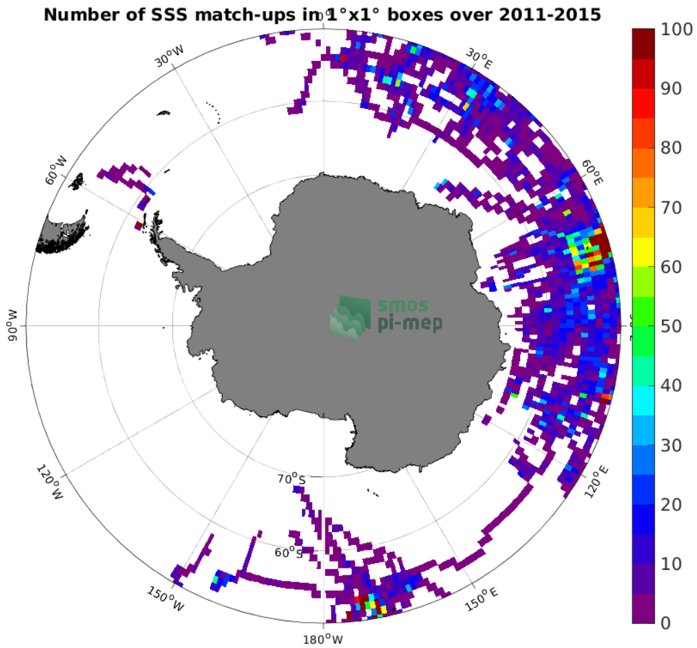
Figure 4: Number of SSS match-ups between Marine mammals SSS and the Aquarius SSS L3 OR v5 - 7-Day running - Rain mask (NASA-GSFC) SSS product for the Southern Ocean Pi-MEP region over 1^{\circ} \times 1^{\circ} boxes and for the full satellite product period.
