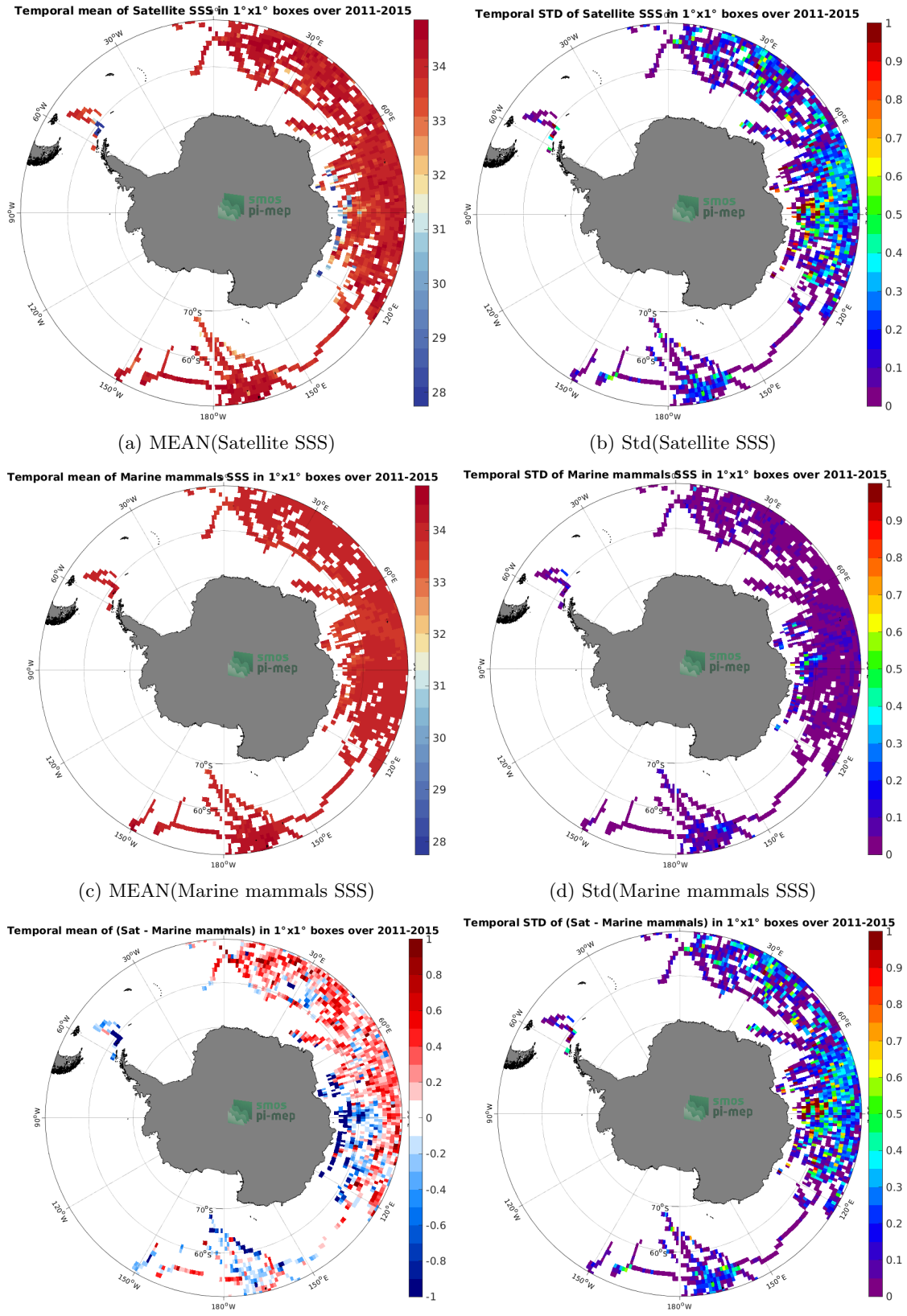
Figure 6: Temporal mean (left) and Std (right) of SSS from Aquarius SSS L3 OR v5 - 7-Day running - Rain mask (NASA-GSFC) (top), Marine mammals (middle), and of \Delta SSS (Satellite - Marine mammals). Only match-up pairs are used to generate these maps.
