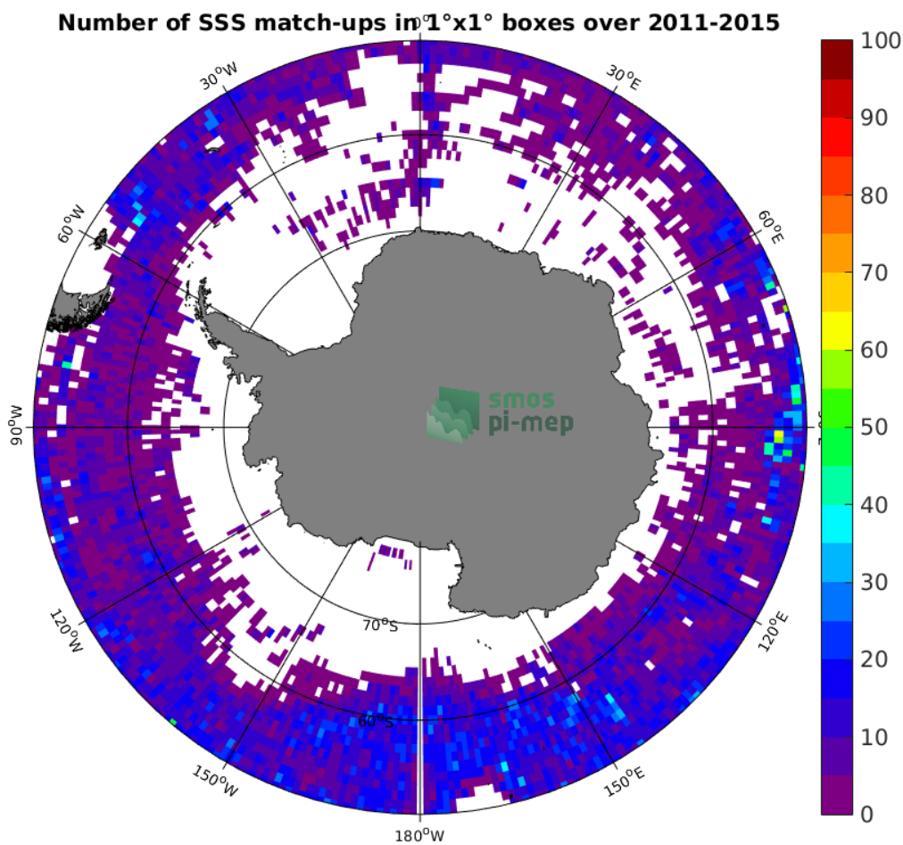
Figure 4: Number of SSS match-ups between Argo SSS and the Aquarius-L3-OR-V5-7DAY-RUNNING-RAIN-MASK-1DEG SSS product for the Southern Ocean Pi-MEP region over 1^{\circ} \times 1^{\circ} boxes and for the full satellite product period.
