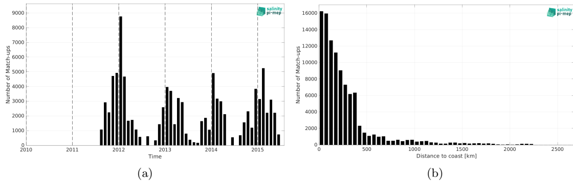
Figure 2: Number of match-ups between TSG (SAMOS) and Aquarius SSS L3 OR v5 - Monthly (NASA-GSFC) SSS as a function of time (a) and as function of the distance to coast (b) over the Southern Ocean Pi-MEP region and for the full satellite product period.
