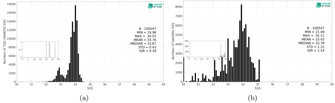
Figure 3: Histograms of SSS from TSG (SAMOS) (a) and Aquarius SSS L3 OR v5 - Monthly (NASA-GSFC) (b) considering all match-up pairs per bins of 0.1 over the Southern Ocean Pi-MEP region and for the full satellite product period.
