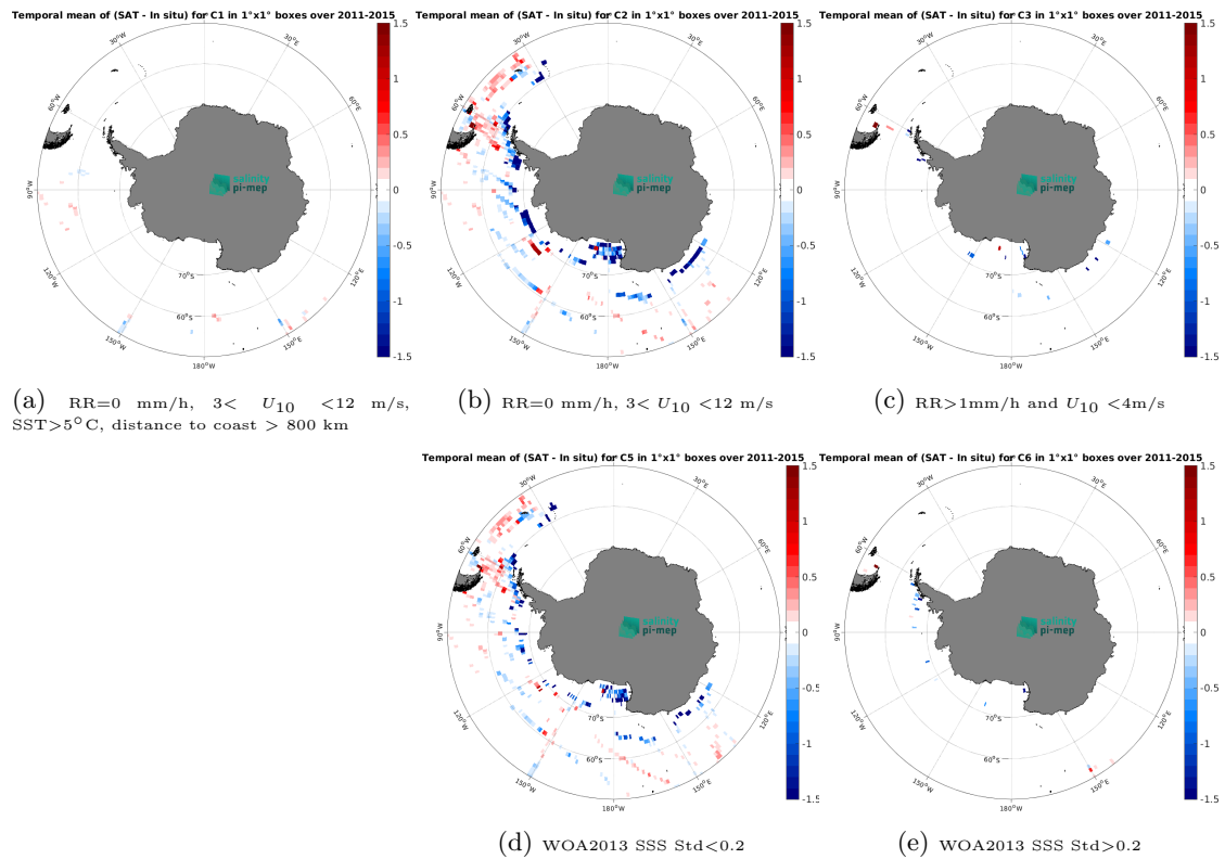
Figure 14: Temporal mean gridded over spatial boxes of size 1^\circ \times 1^\circ of \Delta\text{SSS} (Aquarius SSS L3 OR v5 - Monthly (NASA-GSFC) - TSG (SAMOS)) for 5 different subdatasets corresponding to: RR=0 mm/h, 3 < U_{10} < 12 m/s, SST > 5°C, distance to coast > 800 km (a), RR=0 mm/h, 3 < U_{10} < 12 m/s (b), RR > 1mm/h and U_{10} < 4 m/s (c), WOA2013 SSS Std < 0.2 (d), WOA2013 SSS Std > 0.2 (e).
