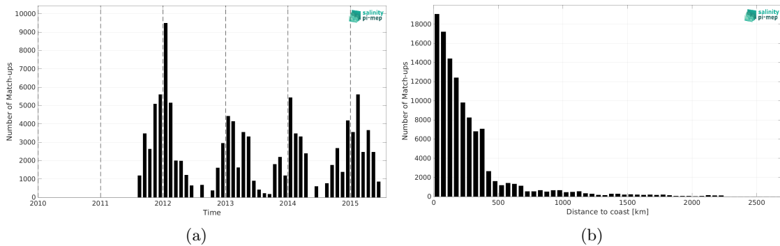
Figure 1: Number of match-ups between TSG (SAMOS) and Aquarius SSS L3 OR v5 - Monthly (NASA-GSFC) SSS as a function of time (a) and as function of the distance to coast (b) over the Southern Ocean Pi-MEP region and for the full satellite product period.
