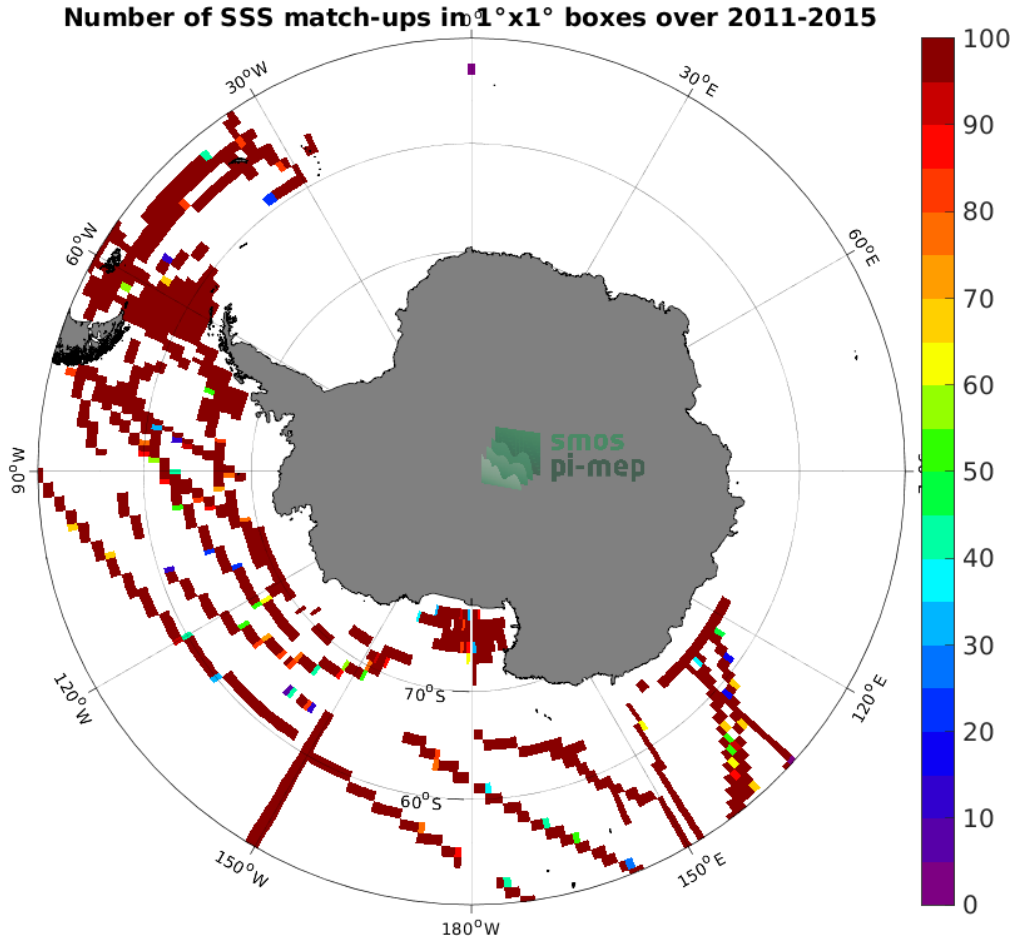
Figure 4: Number of SSS match-ups between TSG (SAMOS) SSS and the Aquarius SSS L3 OR v5 - Monthly (NASA-GSFC) SSS product for the Southern Ocean Pi-MEP region over 1^\circ \times 1^\circ boxes and for the full satellite product period.
