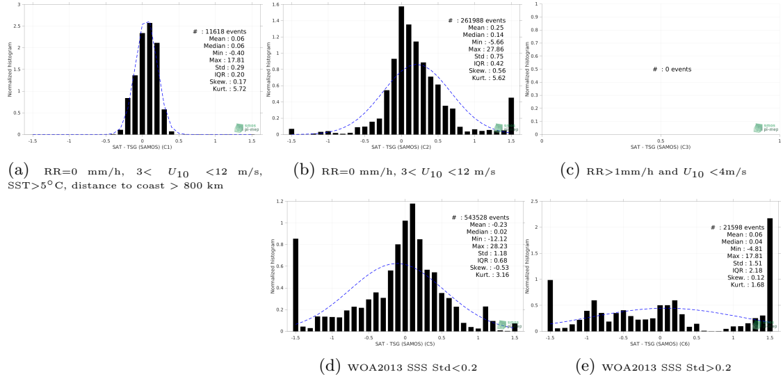
Figure 13: Normalized histogram of \Delta SSS (Aquarius SSS L3 OR v5 - Monthly (NASA-GSFC) - TSG (SAMOS)) for 5 different subdatasets corresponding to: RR=0 mm/h, 3 < U_{10} < 12 m/s, SST > 5°C, distance to coast > 800 km (a), RR=0 mm/h, 3 < U_{10} < 12 m/s (b), RR > 1mm/h and U_{10} < 4 m/s (c), WOA2013 SSS Std < 0.2 (d), WOA2013 SSS Std > 0.2 (e).
