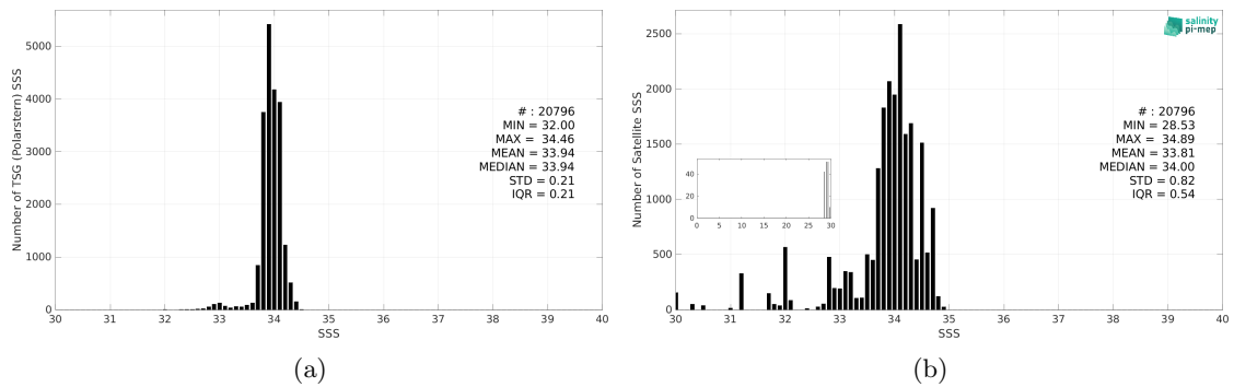
Figure 3: Histograms of SSS from TSG (Polarstern) (a) and Aquarius SSS L3 OR v5 - Monthly (NASA-GSFC) (b) considering all match-up pairs per bins of 0.1 over the Southern Ocean Pi-MEP region and for the full satellite product period.
