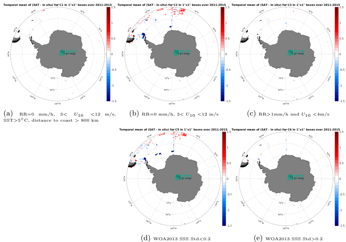
Figure 14: Temporal mean gridded over spatial boxes of size 1^\circ \times 1^\circ of \Delta SSS (Aquarius SSS L3 OR v5 - Monthly (NASA-GSFC) - TSG (Polarstern)) for 5 different subdatasets corresponding to: RR=0 mm/h, 3 < U_{10} < 12 m/s, SST > 5^\circ\text{C} , distance to coast > 800 km (a), RR=0 mm/h, 3 < U_{10} < 12 m/s (b), RR > 1 mm/h and U_{10} < 4 m/s (c), WOA2013 SSS Std < 0.2 (d), WOA2013 SSS Std > 0.2 (e).
