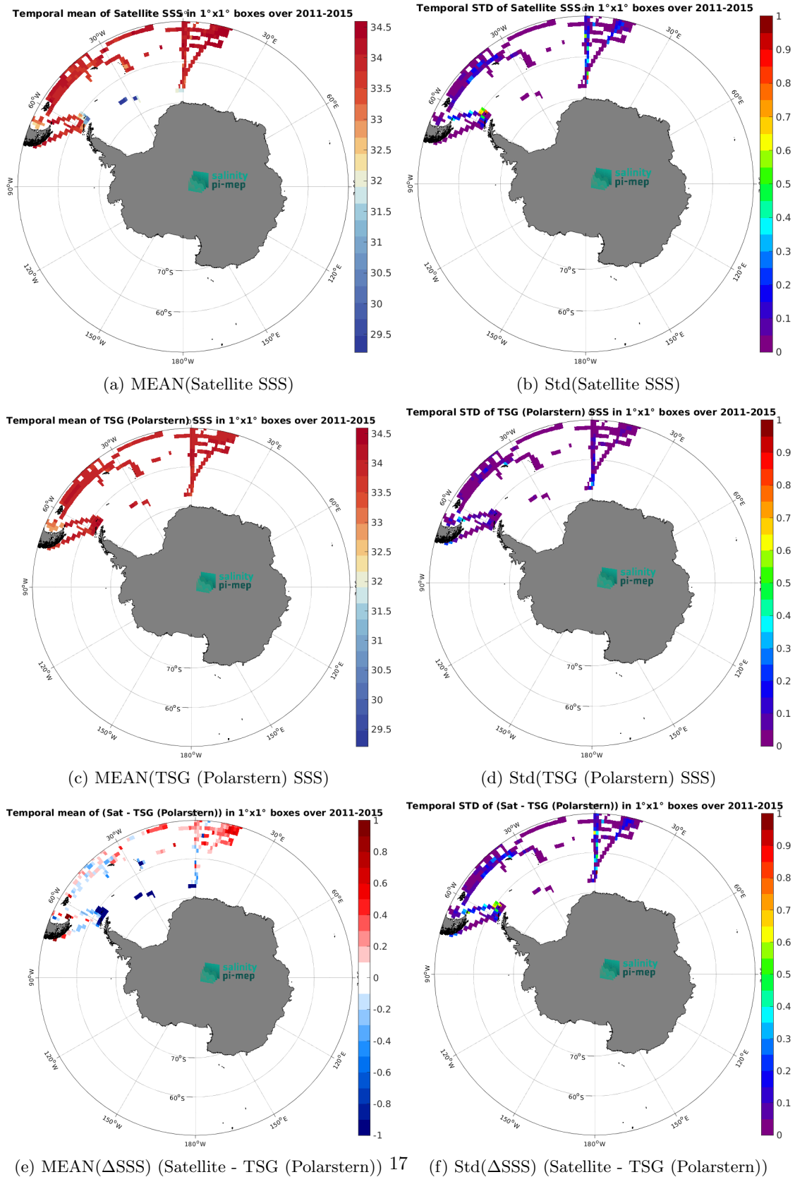
Figure 7: Temporal mean (left) and Std (right) of SSS from Aquarius SSS L3 OR v5 - Monthly (NASA-GSFC) (top), TSG (Polarstern) (middle), and of \Delta SSS (Satellite - TSG (Polarstern)). Only match-up pairs are used to generate these maps.
