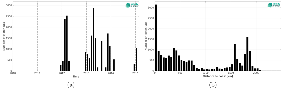
Figure 2: Number of match-ups between TSG (Polarstern) and Aquarius SSS L3 OR v5 - Monthly (NASA-GSFC) SSS as a function of time (a) and as function of the distance to coast (b) over the Southern Ocean Pi-MEP region and for the full satellite product period.
