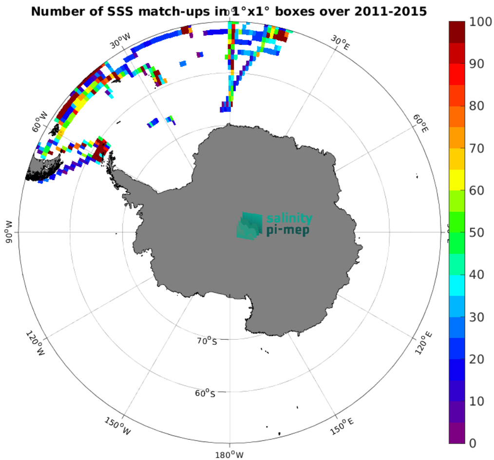
Figure 4: Number of SSS match-ups between TSG (Polarstern) SSS and the Aquarius SSS L3 OR v5 - Monthly (NASA-GSFC) SSS product for the Southern Ocean Pi-MEP region over 1^\circ \times 1^\circ boxes and for the full satellite product period.
