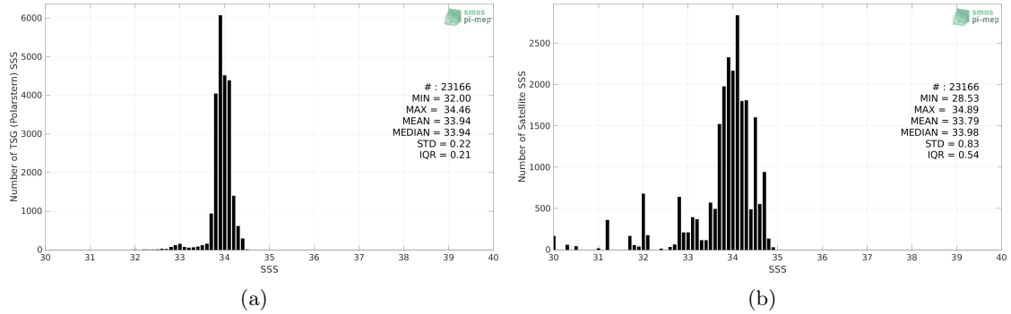
Figure 2: Histograms of SSS from TSG (Polarstern) (a) and Aquarius SSS L3 OR v5 - Monthly (NASA-GSFC) (b) considering all match-up pairs per bins of 0.1 over the Southern Ocean Pi-MEP region and for the full satellite product period.
