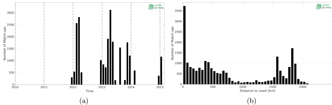
Figure 1: Number of match-ups between TSG (Polarstern) and Aquarius SSS L3 OR v5 - Monthly (NASA-GSFC) SSS as a function of time (a) and as function of the distance to coast (b) over the Southern Ocean Pi-MEP region and for the full satellite product period.
