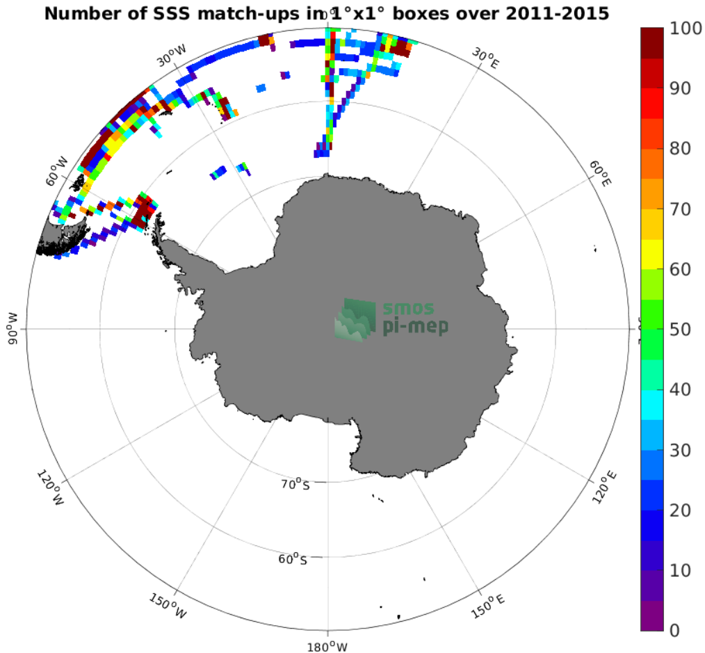
Figure 4: Number of SSS match-ups between TSG (Polarstern) SSS and the Aquarius SSS L3 OR v5 - Monthly (NASA-GSFC) SSS product for the Southern Ocean Pi-MEP region over 1^\circ \times 1^\circ boxes and for the full satellite product period.
