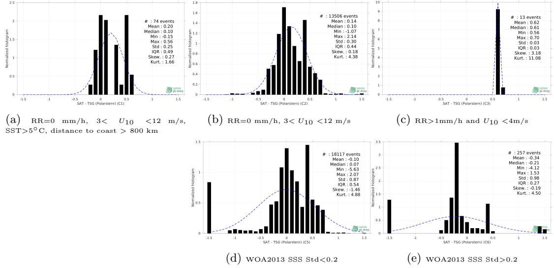
Figure 13: Normalized histogram of \Delta SSS (Aquarius SSS L3 OR v5 - Monthly (NASA-GSFC) - TSG (Polarstern)) for 5 different subdatasets corresponding to: RR=0 mm/h, 3 < U_{10} < 12 m/s, SST > 5°C, distance to coast > 800 km (a), RR=0 mm/h, 3 < U_{10} < 12 m/s (b), RR > 1mm/h and U_{10} < 4 m/s (c), WOA2013 SSS Std < 0.2 (d), WOA2013 SSS Std > 0.2 (e).
