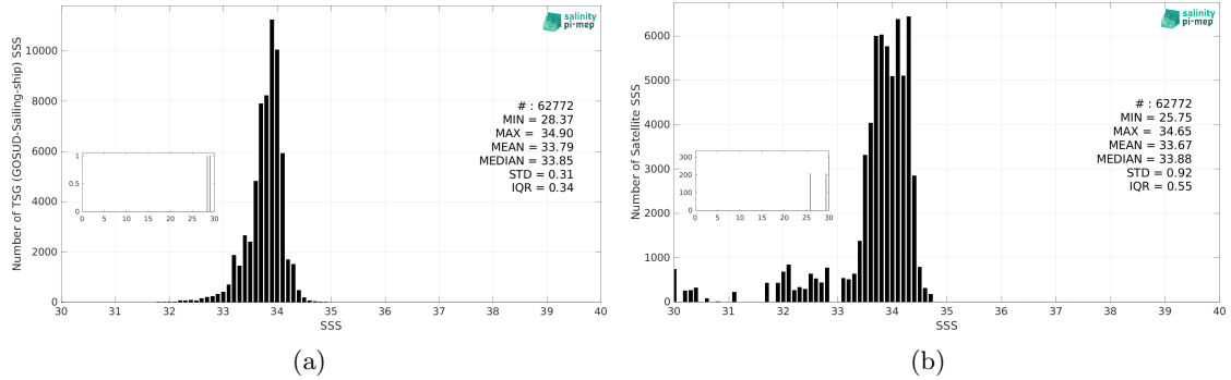
Figure 3: Histograms of SSS from TSG (GOSUD-Sailing-ship) (a) and Aquarius SSS L3 OR v5 - Monthly (NASA-GSFC) (b) considering all match-up pairs per bins of 0.1 over the Southern Ocean Pi-MEP region and for the full satellite product period.
