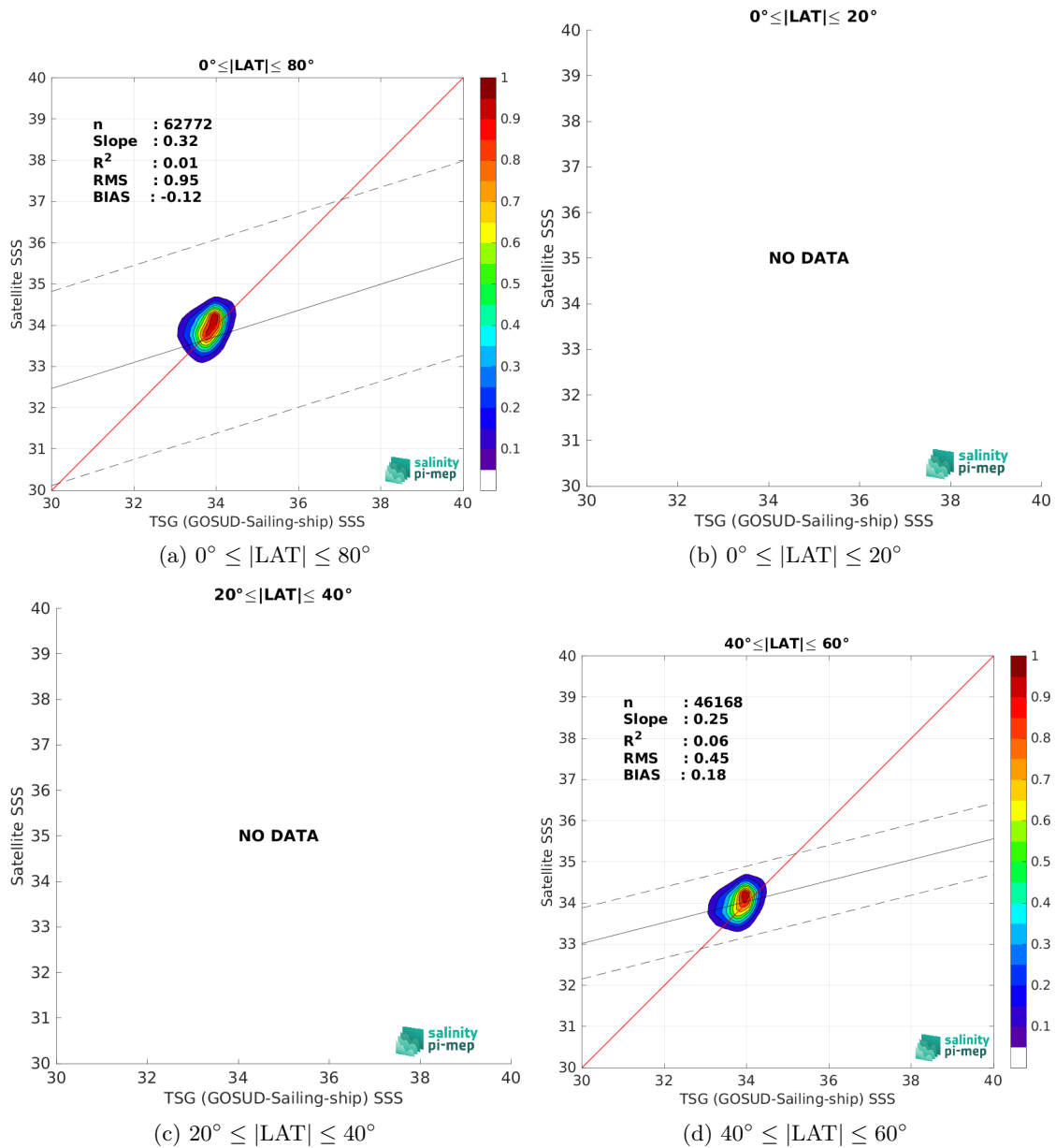
Figure 10: Contour maps of the concentration of Aquarius SSS L3 OR v5 - Monthly (NASA-GSFC) SSS (y-axis) versus TSG (GOSUD-Sailing-ship) SSS (x-axis) at match-up pairs for different latitude bands. For each plot, the red line shows x=y . The black thin and dashed lines indicate a linear fit through the data cloud and the \pm 95\% confidence levels, respectively. The number match-up pairs n , the slope and R^2 coefficient of the linear fit, the root mean square (RMS) and the mean bias between satellite and in situ data are indicated for each latitude band in each plots.
