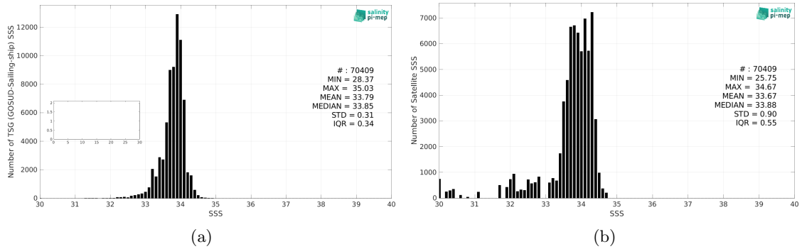
Figure 2: Histograms of SSS from TSG (GOSUD-Sailing-ship) (a) and Aquarius SSS L3 OR v5 - Monthly (NASA-GSFC) (b) considering all match-up pairs per bins of 0.1 over the Southern Ocean Pi-MEP region and for the full satellite product period.
