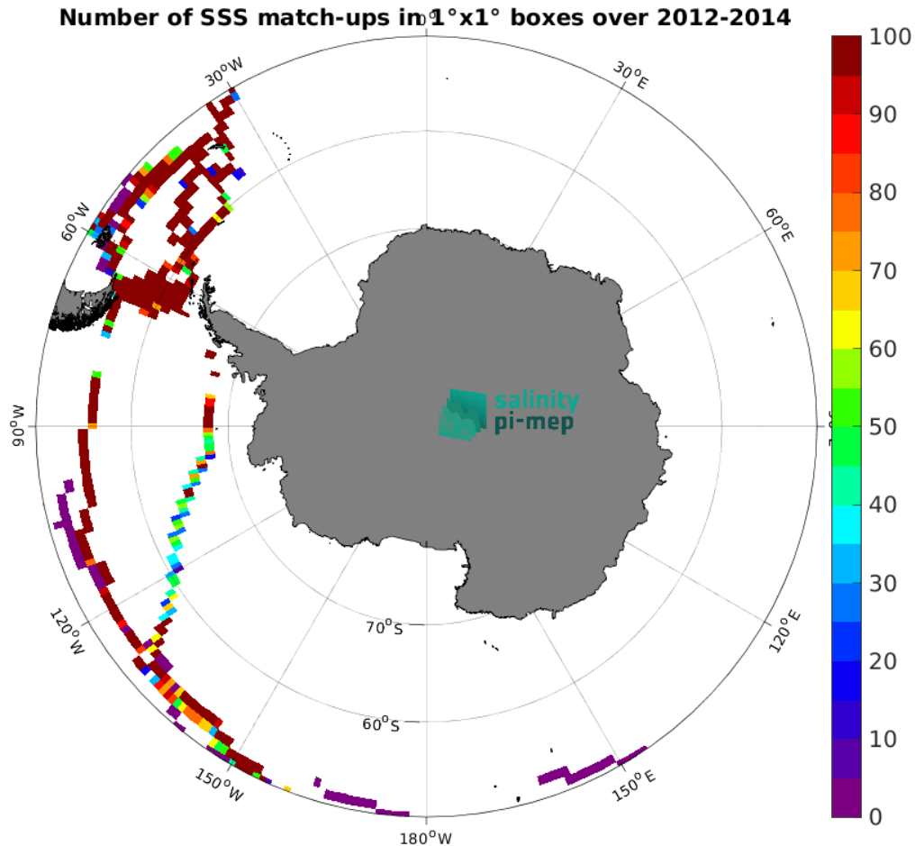
Figure 4: Number of SSS match-ups between TSG (GOSUD-Sailing-ship) SSS and the Aquarius SSS L3 OR v5 - Monthly (NASA-GSFC) SSS product for the Southern Ocean Pi-MEP region over 1^\circ \times 1^\circ boxes and for the full satellite product period.
