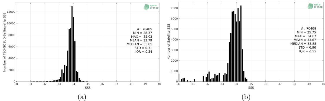
Figure 2: Histograms of SSS from TSG-GOSUD-Sailing-ship (a) and Aquarius-L3-OR-V5-MONTHLY-1DEG (b) considering all match-up pairs per bins of 0.1 over the Southern Ocean Pi-MEP region and for the full satellite product period.
