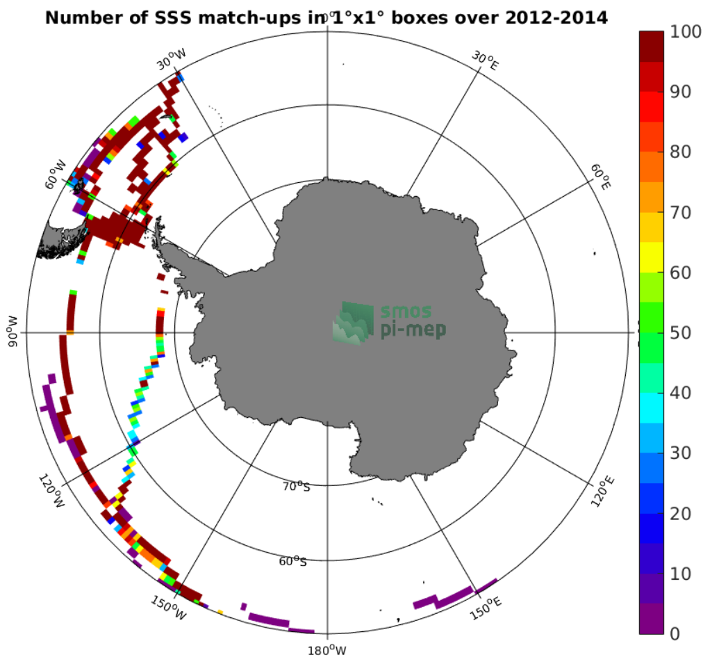
Figure 4: Number of SSS match-ups between TSG-GOSUD-Sailing-ship SSS and the Aquarius-L3-OR-V5-MONTHLY-1DEG SSS product for the Southern Ocean Pi-MEP region over 1°x1° boxes and for the full satellite product period.
