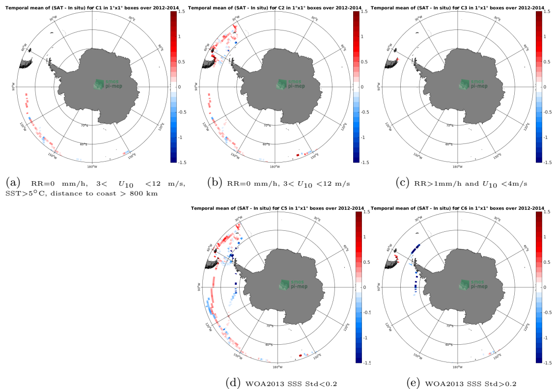
Figure 12: Temporal mean gridded over spatial boxes of size 1^\circ \times 1^\circ of \Delta SSS (Aquarius-L3-OR-V5-MONTHLY-1DEG - TSG-GOSUD-Sailing-ship) for 5 different subdatasets corresponding to: RR=0 mm/h, 3 < U_{10} < 12 m/s, SST > 5°C, distance to coast > 800 km (a), RR=0 mm/h, 3 < U_{10} < 12 m/s (b), RR > 1mm/h and U_{10} < 4 m/s (c), WOA2013 SSS Std < 0.2 (d), WOA2013 SSS Std > 0.2 (e).
