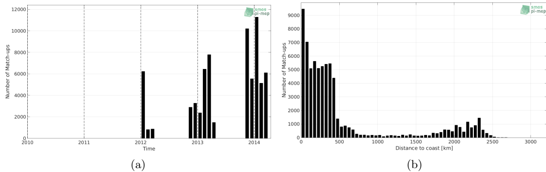
Figure 1: Number of match-ups between TSG-GOSUD-Sailing-ship and Aquarius-L3-OR-V5-MONTHLY-1DEG SSS as a function of time (a) and as function of the distance to coast (b) over the Southern Ocean Pi-MEP region and for the full satellite product period.
