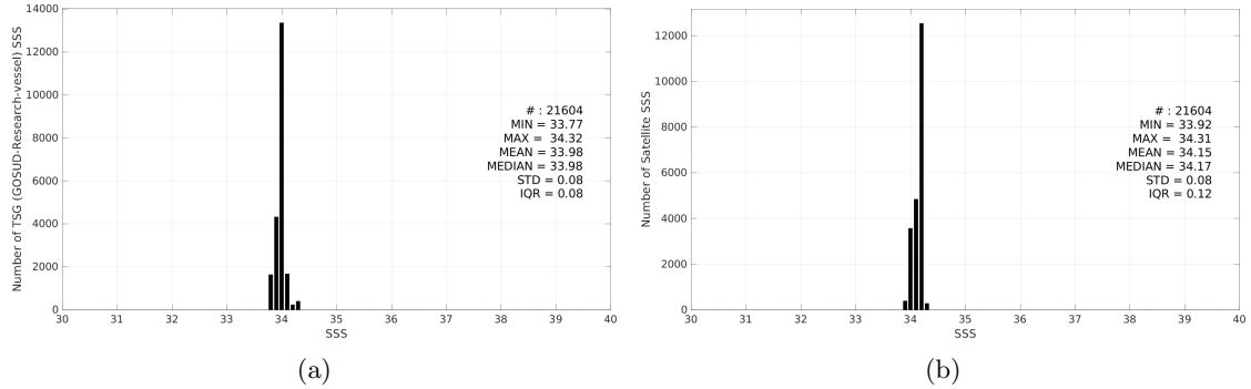
Figure 3: Histograms of SSS from TSG (GOSUD-Research-vessel) (a) and Aquarius SSS L3 OR v5 - Monthly (NASA-GSFC) (b) considering all match-up pairs per bins of 0.1 over the Southern Ocean Pi-MEP region and for the full satellite product period.
