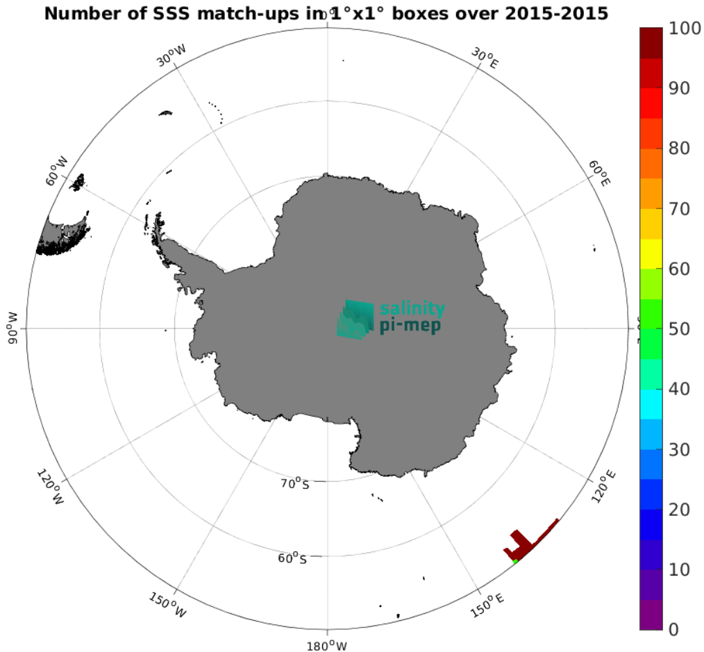
Figure 5: Number of SSS match-ups between TSG (GOSUD-Research-vessel) SSS and the Aquarius SSS L3 OR v5 - Monthly (NASA-GSFC) SSS product for the Southern Ocean Pi-MEP region over 1^\circ \times 1^\circ boxes and for the full satellite product period.
