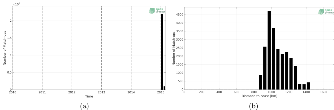
Figure 1: Number of match-ups between TSG (GOSUD-Research-vessel) and Aquarius SSS L3 OR v5 - Monthly (NASA-GSFC) SSS as a function of time (a) and as function of the distance to coast (b) over the Southern Ocean Pi-MEP region and for the full satellite product period.
