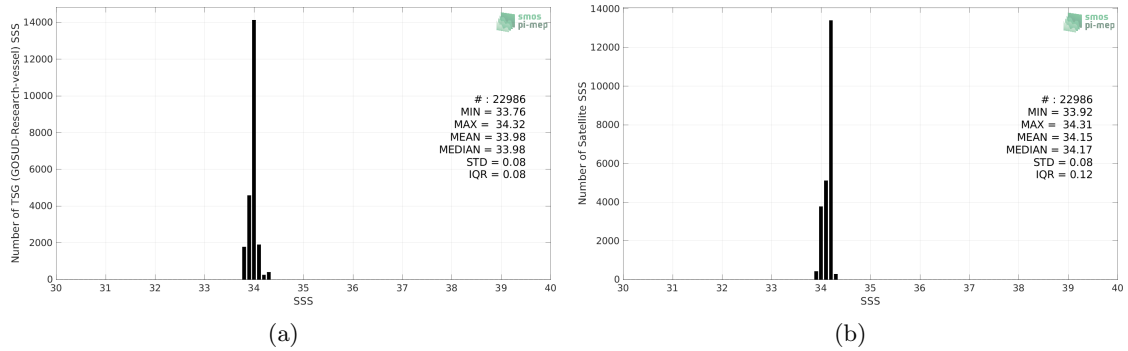
Figure 2: Histograms of SSS from TSG (GOSUD-Research-vessel) (a) and Aquarius SSS L3 OR v5 - Monthly (NASA-GSFC) (b) considering all match-up pairs per bins of 0.1 over the Southern Ocean Pi-MEP region and for the full satellite product period.
