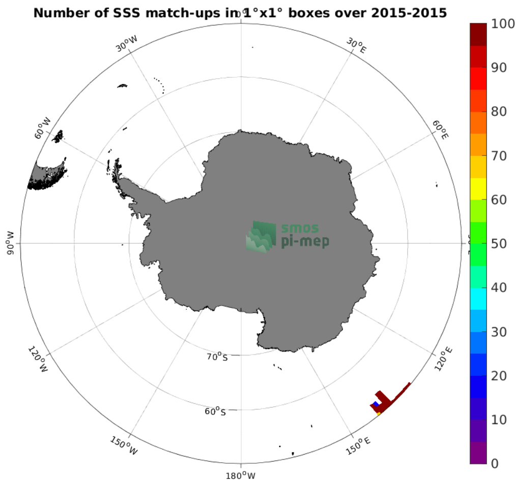
Figure 4: Number of SSS match-ups between TSG (GOSUD-Research-vessel) SSS and the Aquarius SSS L3 OR v5 - Monthly (NASA-GSFC) SSS product for the Southern Ocean Pi-MEP region over 1^{\circ} \times 1^{\circ} boxes and for the full satellite product period.
