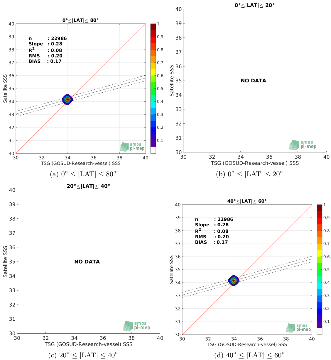
Figure 9: Contour maps of the concentration of Aquarius SSS L3 OR v5 - Monthly (NASA-GSFC) SSS ( y -axis) versus TSG (GOSUD-Research-vessel) SSS ( x -axis) at match-up pairs for different latitude bands. For each plot, the red line shows x=y . The black thin and dashed lines indicate a linear fit through the data cloud and the \pm 95\% confidence levels, respectively. The number match-up pairs n , the slope and R^2 coefficient of the linear fit, the root mean square (RMS) and the mean bias between satellite and in situ data are indicated for each latitude band in each plots.
