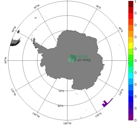
(f) Std( \Delta SSS) (Satellite - TSG (GOSUD-Research-vessel))
