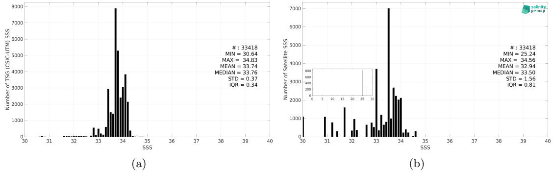
Figure 3: Histograms of SSS from TSG (CSIC-UTM) (a) and Aquarius SSS L3 OR v5 - Monthly (NASA-GSFC) (b) considering all match-up pairs per bins of 0.1 over the Southern Ocean Pi-MEP region and for the full satellite product period.
