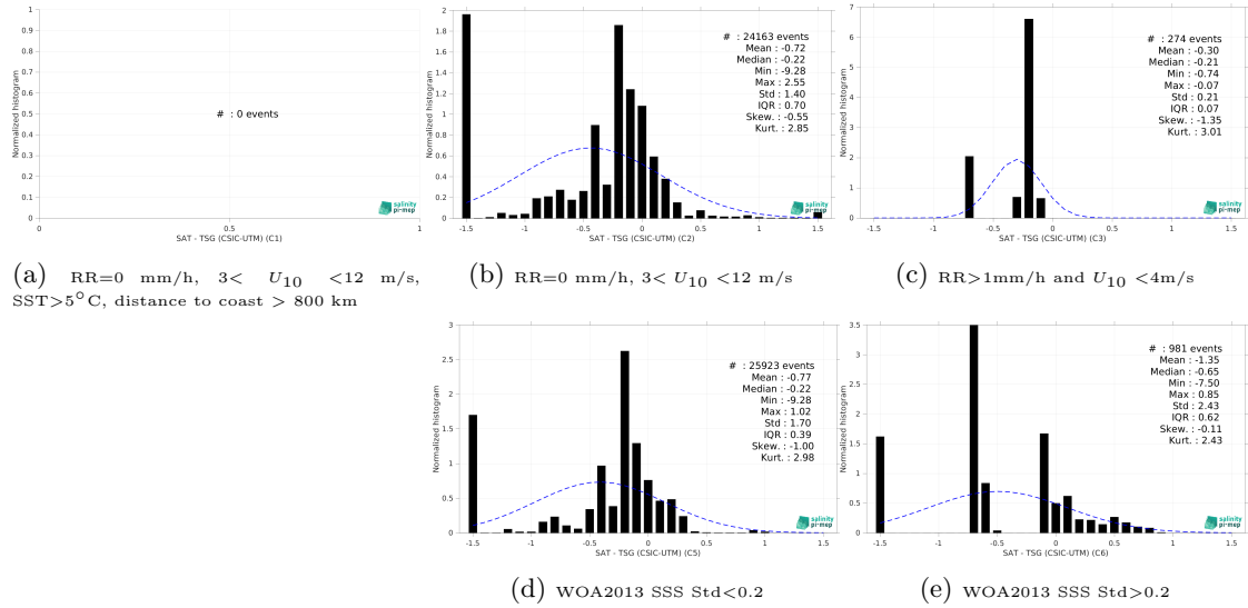
Figure 15: Normalized histogram of \Delta\text{SSS} (Aquarius SSS L3 OR v5 - Monthly (NASA-GSFC) - TSG (CSIC-UTM)) for 5 different subdatasets corresponding to: RR=0 mm/h, 3 < U_{10} < 12 m/s, SST > 5^\circ\text{C} , distance to coast > 800 km (a), RR=0 mm/h, 3 < U_{10} < 12 m/s (b), RR > 1\text{mm/h} and U_{10} < 4\text{m/s} (c), WOA2013 SSS Std < 0.2 (d), WOA2013 SSS Std > 0.2 (e).
