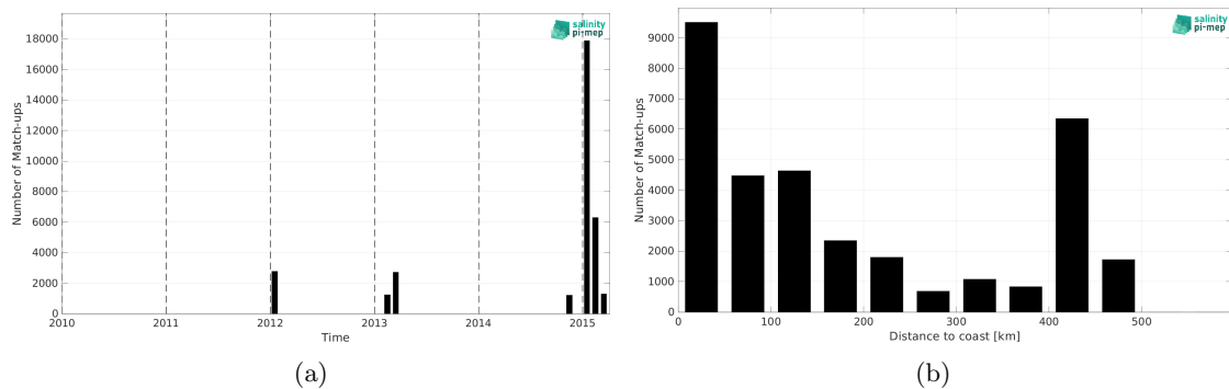
Figure 2: Number of match-ups between TSG (CSIC-UTM) and Aquarius SSS L3 OR v5 - Monthly (NASA-GSFC) SSS as a function of time (a) and as function of the distance to coast (b) over the Southern Ocean Pi-MEP region and for the full satellite product period.
