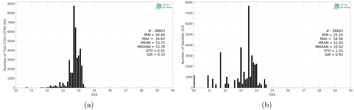
Figure 2: Histograms of SSS from TSG (CSIC-UTM) (a) and Aquarius SSS L3 OR v5 - Monthly (NASA-GSFC) (b) considering all match-up pairs per bins of 0.1 over the Southern Ocean Pi-MEP region and for the full satellite product period.
