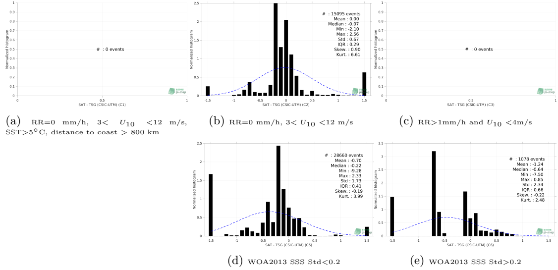
Figure 13: Normalized histogram of \Delta SSS (Aquarius SSS L3 OR v5 - Monthly (NASA-GSFC) - TSG (CSIC-UTM)) for 5 different subdatasets corresponding to: RR=0 mm/h, 3 < U_{10} < 12 m/s, SST > 5°C, distance to coast > 800 km (a), RR=0 mm/h, 3 < U_{10} < 12 m/s (b), RR > 1mm/h and U_{10} < 4 m/s (c), WOA2013 SSS Std < 0.2 (d), WOA2013 SSS Std > 0.2 (e).
