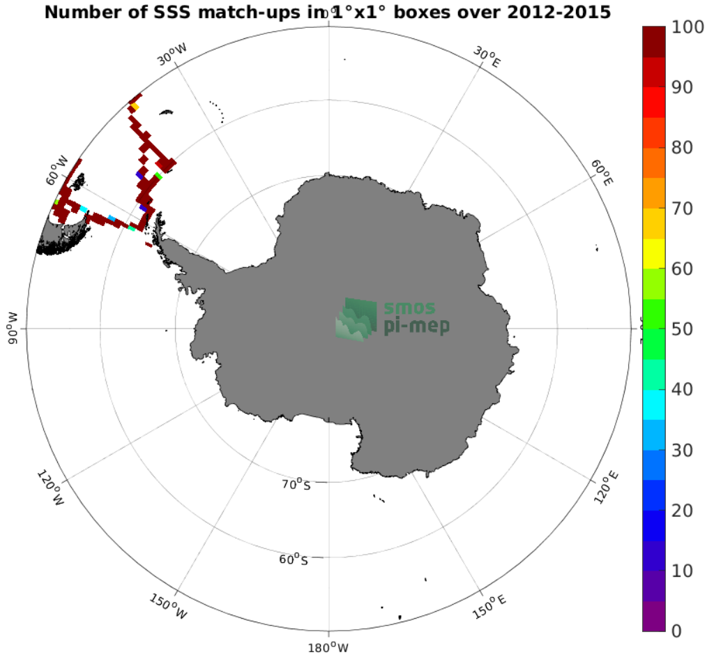
Figure 4: Number of SSS match-ups between TSG (CSIC-UTM) SSS and the Aquarius SSS L3 OR v5 - Monthly (NASA-GSFC) SSS product for the Southern Ocean Pi-MEP region over 1^\circ \times 1^\circ boxes and for the full satellite product period.
