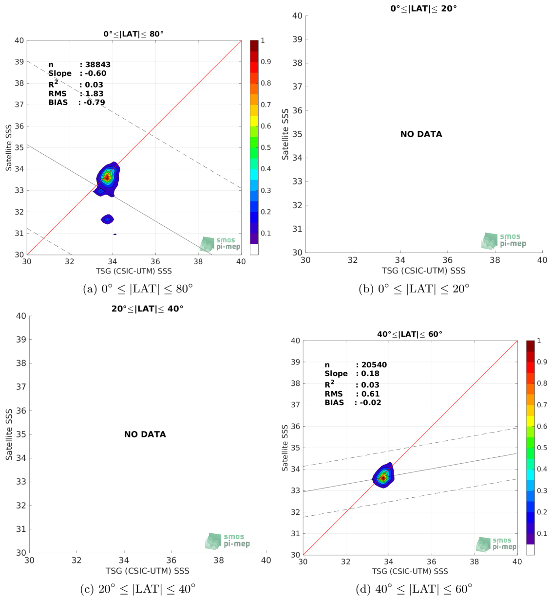
Figure 9: Contour maps of the concentration of Aquarius SSS L3 OR v5 - Monthly (NASA-GSFC) SSS (y-axis) versus TSG (CSIC-UTM) SSS (x-axis) at match-up pairs for different latitude bands. For each plot, the red line shows x=y . The black thin and dashed lines indicate a linear fit through the data cloud and the \pm 95\% confidence levels, respectively. The number match-up pairs n , the slope and R^2 coefficient of the linear fit, the root mean square (RMS) and the mean bias between satellite and in situ data are indicated for each latitude band in each plot.
