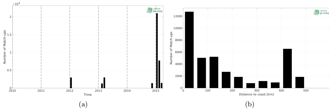
Figure 1: Number of match-ups between TSG (CSIC-UTM) and Aquarius SSS L3 OR v5 - Monthly (NASA-GSFC) SSS as a function of time (a) and as function of the distance to coast (b) over the Southern Ocean Pi-MEP region and for the full satellite product period.
