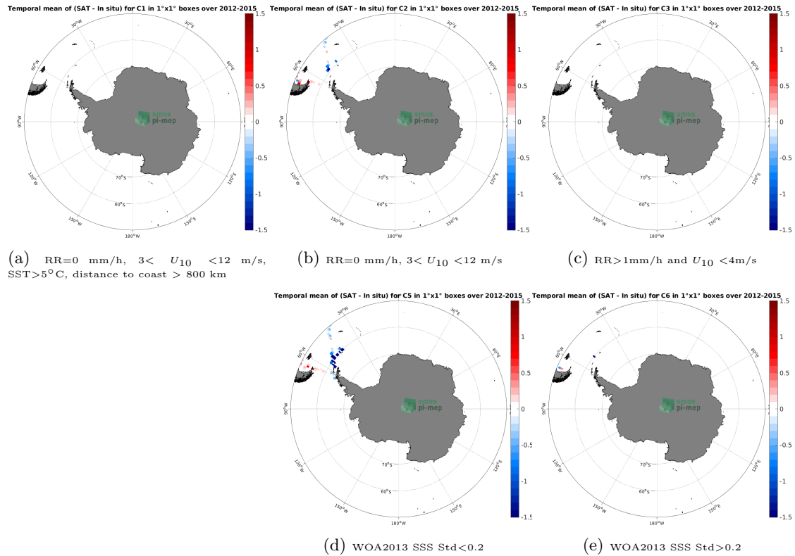
Figure 12: Temporal mean gridded over spatial boxes of size 1^{\circ}\times 1^{\circ} of \Delta\text{SSS} (Aquarius SSS L3 OR v5 - Monthly (NASA-GSFC) - TSG (CSIC-UTM)) for 5 different subdatasets corresponding to:RR=0 mm/h, 3 < U_{10} < 12 m/s, SST >5^{\circ}\text{C} , distance to coast > 800 km (a), RR=0 mm/h, 3 < U_{10} < 12 m/s (b), RR >1 mm/h and U_{10} < 4 m/s (c), WOA2013 SSS Std <0.2 (d), WOA2013 SSS Std >0.2 (e).
