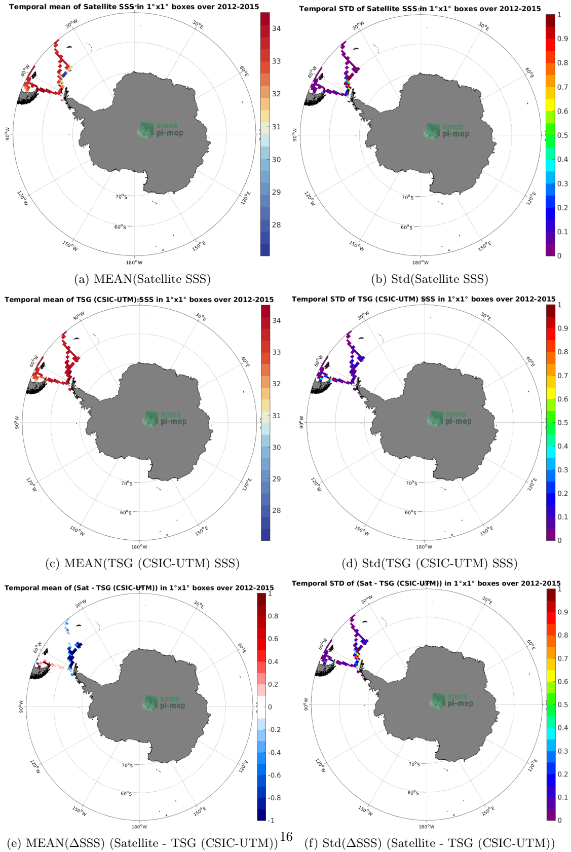
Figure 6: Temporal mean (left) and Std (right) of SSS from Aquarius SSS L3 OR v5 - Monthly (NASA-GSFC) (top), TSG (CSIC-UTM) (middle), and of \Delta SSS (Satellite - TSG (CSIC-UTM)). Only match-up pairs are used to generate these maps.
