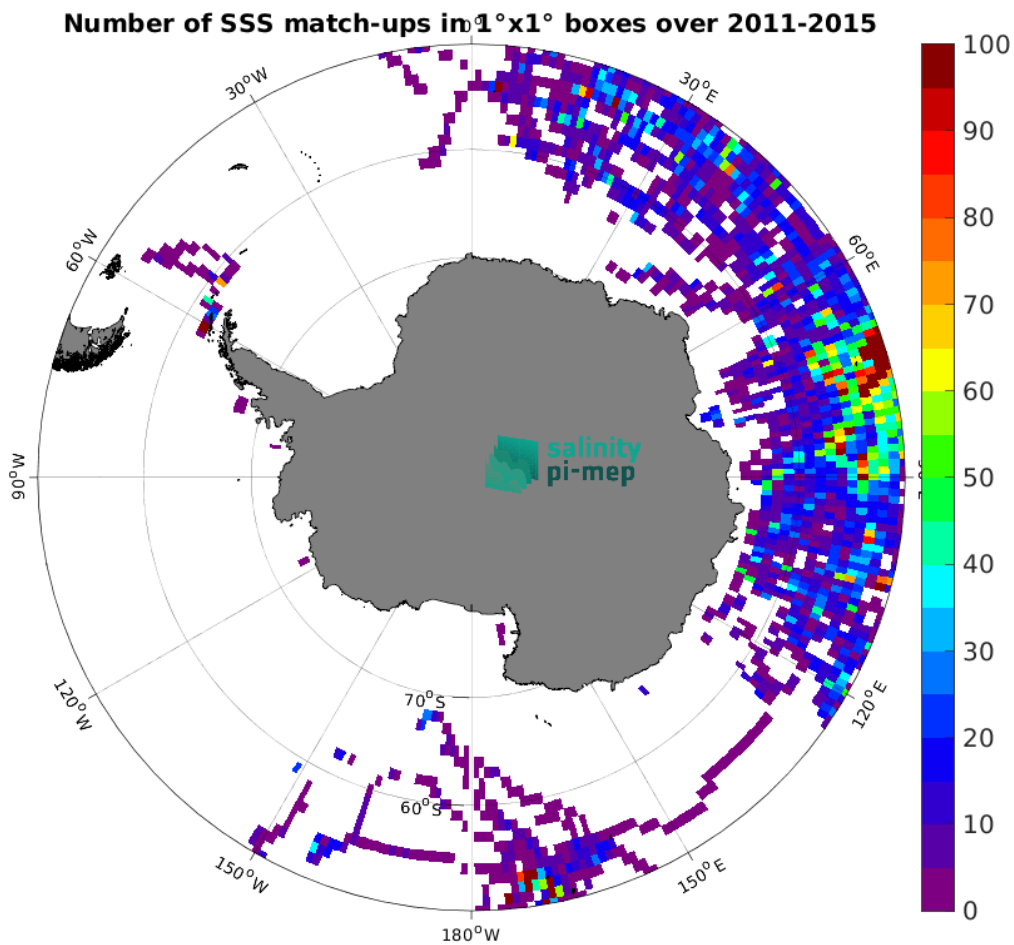
Figure 5: Number of SSS match-ups between Marine mammals SSS and the Aquarius SSS L3 OR v5 - Monthly (NASA-GSFC) SSS product for the Southern Ocean Pi-MEP region over 1^{\circ} \times 1^{\circ} boxes and for the full satellite product period.
