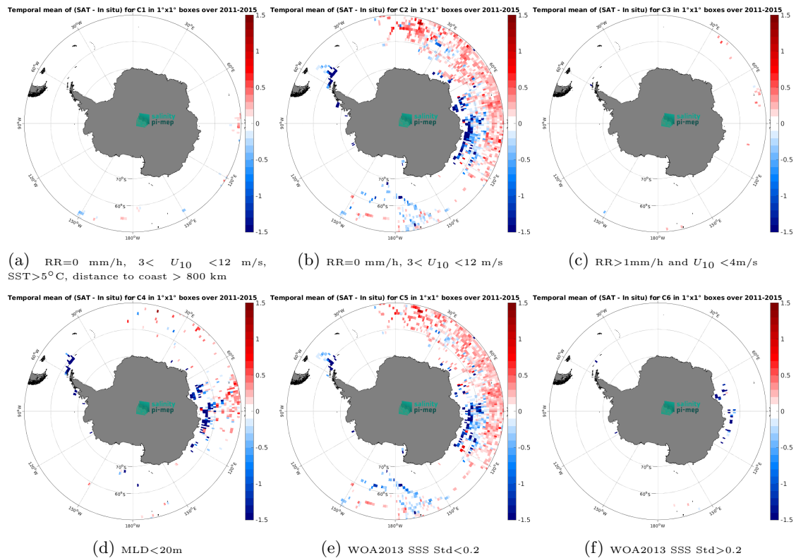
Figure 14: Temporal mean gridded over spatial boxes of size 1^\circ \times 1^\circ of \Delta SSS (Aquarius SSS L3 OR v5 - Monthly (NASA-GSFC) - Marine mammals) for 6 different subdatasets corresponding to:RR=0 mm/h, 3 < U_{10} < 12 m/s, SST>5°C, distance to coast > 800 km (a), RR=0 mm/h, 3 < U_{10} < 12 m/s (b), RR>1mm/h and U_{10} < 4 m/s (c),MLD<20m (d),WOA2013 SSS Std<0.2 (e),WOA2013 SSS Std>0.2 (f).
