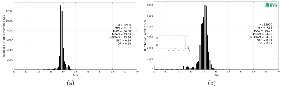
Figure 3: Histograms of SSS from Marine mammals (a) and Aquarius SSS L3 OR v5 - Monthly (NASA-GSFC) (b) considering all match-up pairs per bins of 0.1 over the Southern Ocean Pi-MEP region and for the full satellite product period.
