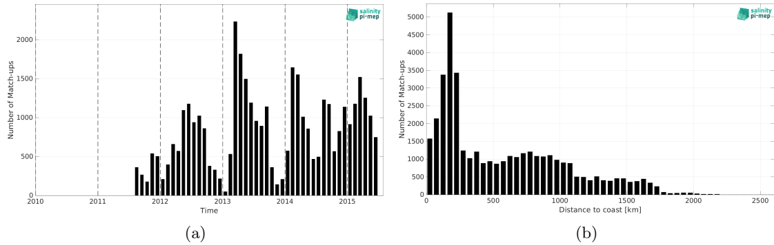
Figure 2: Number of match-ups between Marine mammals and Aquarius SSS L3 OR v5 - Monthly (NASA-GSFC) SSS as a function of time (a) and as function of the distance to coast (b) over the Southern Ocean Pi-MEP region and for the full satellite product period.
