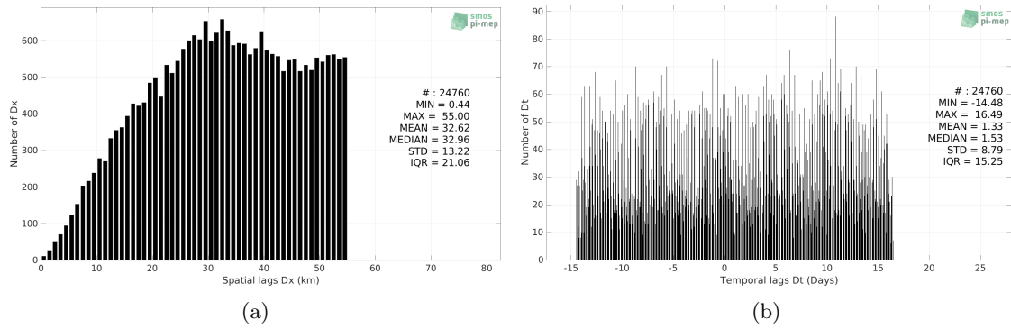
Figure 5: Histograms of the spatial (a) and temporal (b) lags between the location/time of the Marine mammals measurement and the date of the corresponding Aquarius SSS L3 OR v5 - Monthly (NASA-GSFC) SSS pixel.
