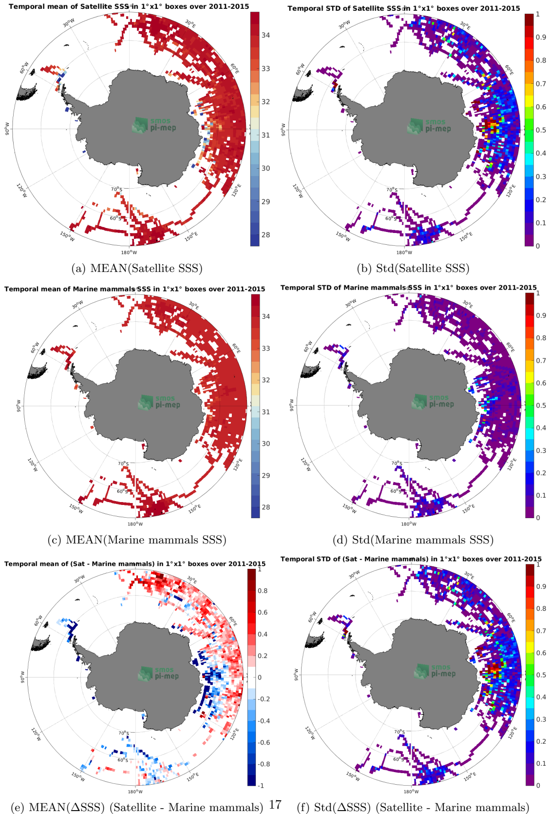
Figure 6: Temporal mean (left) and Std (right) of SSS from Aquarius SSS L3 OR v5 - Monthly (NASA-GSFC) (top), Marine mammals (middle), and of \Delta SSS (Satellite - Marine mammals). Only match-up pairs are used to generate these maps.
