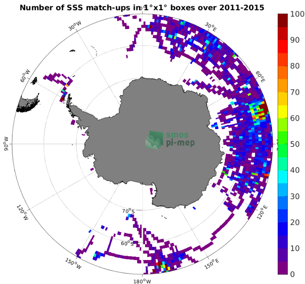
Figure 4: Number of SSS match-ups between Marine mammals SSS and the Aquarius SSS L3 OR v5 - Monthly (NASA-GSFC) SSS product for the Southern Ocean Pi-MEP region over 1^\circ \times 1^\circ boxes and for the full satellite product period.
