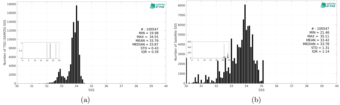
Figure 3: Histograms of SSS from TSG (SAMOS) (a) and Aquarius SSS L3 OR v5 - Monthly - Rain mask (NASA-GSFC) (b) considering all match-up pairs per bins of 0.1 over the Southern Ocean Pi-MEP region and for the full satellite product period.
