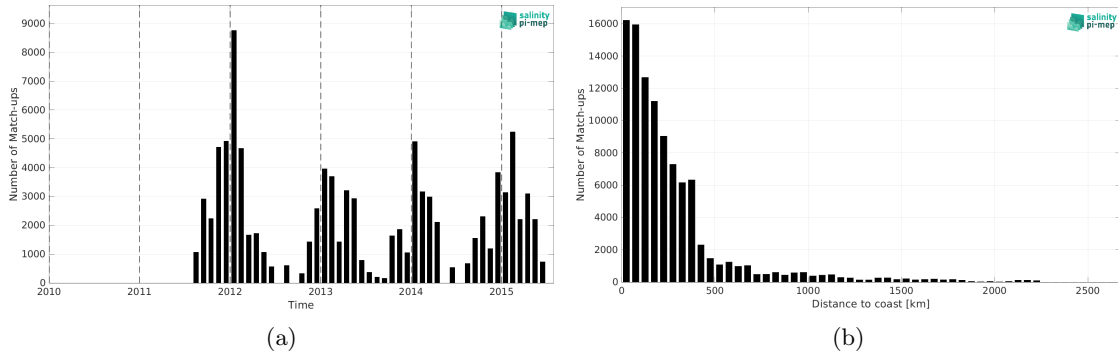
Figure 2: Number of match-ups between TSG (SAMOS) and Aquarius SSS L3 OR v5 - Monthly - Rain mask (NASA-GSFC) SSS as a function of time (a) and as function of the distance to coast (b) over the Southern Ocean Pi-MEP region and for the full satellite product period.
