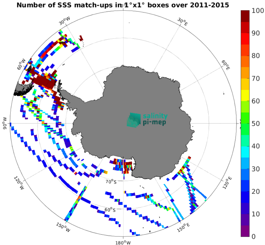
Figure 5: Number of SSS match-ups between TSG (SAMOS) SSS and the Aquarius SSS L3 OR v5 - Monthly - Rain mask (NASA-GSFC) SSS product for the Southern Ocean Pi-MEP region over 1^\circ \times 1^\circ boxes and for the full satellite product period.
