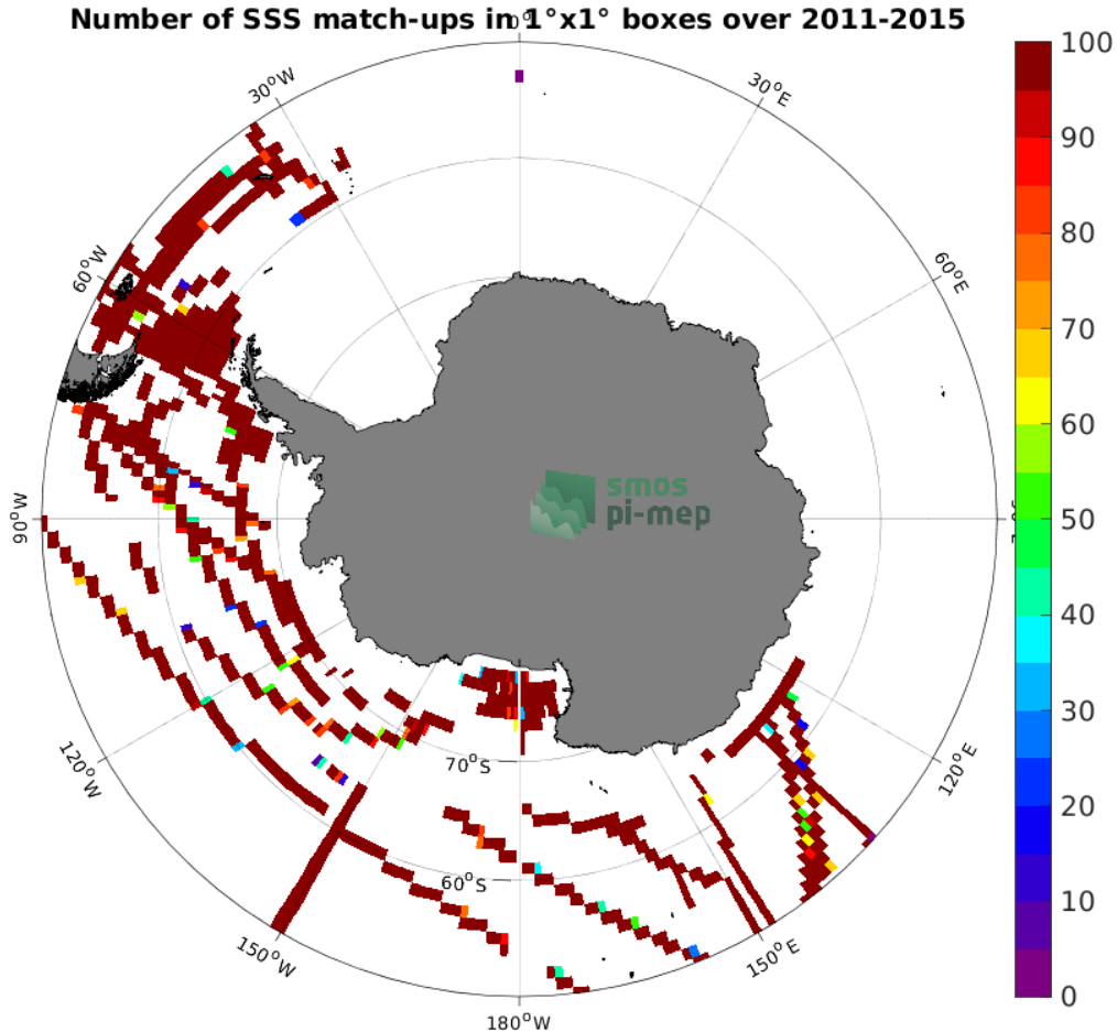
Figure 4: Number of SSS match-ups between TSG (SAMOS) SSS and the Aquarius SSS L3 OR v5 - Monthly - Rain mask (NASA-GSFC) SSS product for the Southern Ocean Pi-MEP region over 1^\circ \times 1^\circ boxes and for the full satellite product period.
