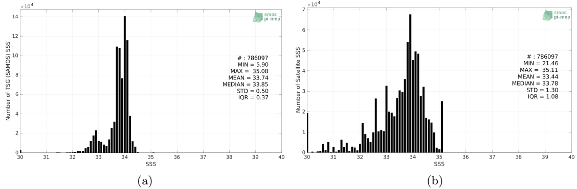
Figure 2: Histograms of SSS from TSG (SAMOS) (a) and Aquarius SSS L3 OR v5 - Monthly - Rain mask (NASA-GSFC) (b) considering all match-up pairs per bins of 0.1 over the Southern Ocean Pi-MEP region and for the full satellite product period.
