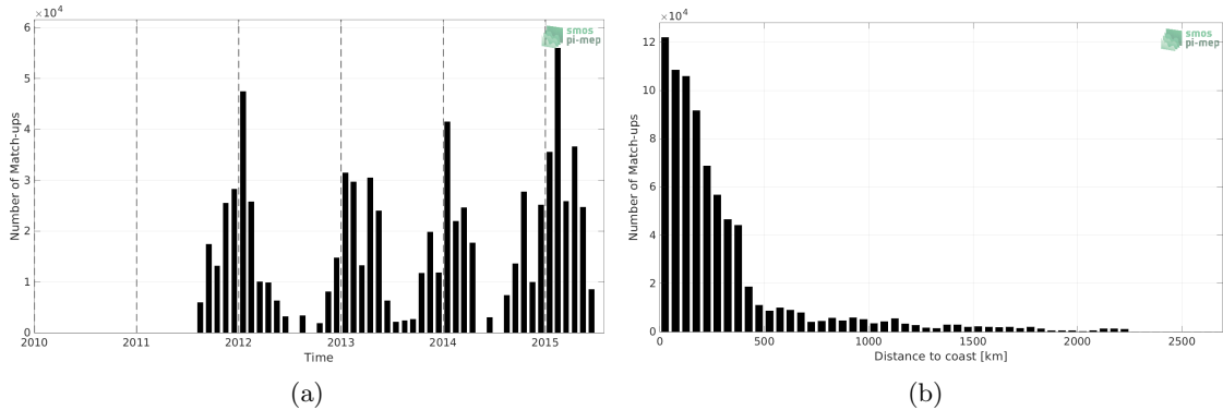
Figure 1: Number of match-ups between TSG (SAMOS) and Aquarius SSS L3 OR v5 - Monthly - Rain mask (NASA-GSFC) SSS as a function of time (a) and as function of the distance to coast (b) over the Southern Ocean Pi-MEP region and for the full satellite product period.
