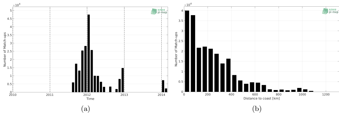
Figure 1: Number of match-ups between TSG-SAMOS and Aquarius-L3-OR-V5-MONTHLY-RAIN-MASK-1DEG SSS as a function of time (a) and as function of the distance to coast (b) over the Southern Ocean Pi-MEP region and for the full satellite product period.
