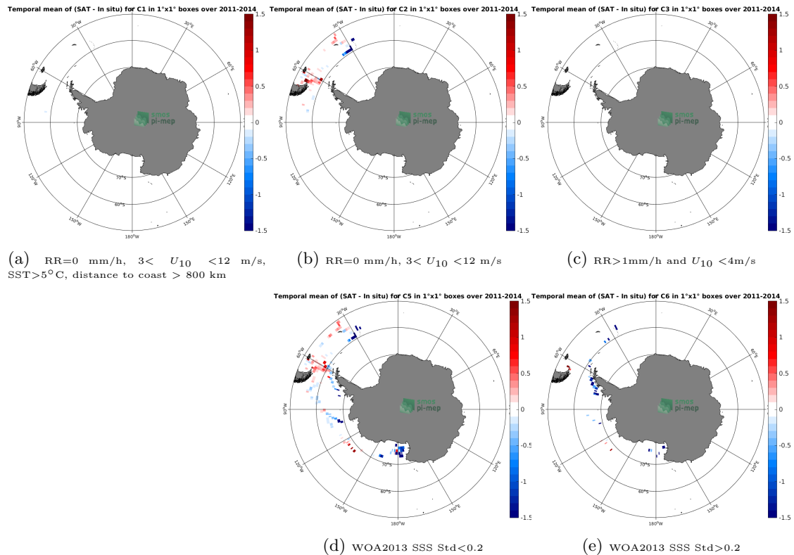
Figure 12: Temporal mean gridded over spatial boxes of size 1^\circ \times 1^\circ of \Delta SSS (Aquarius-L3-OR-V5-MONTHLY-RAIN-MASK-1DEG - TSG-SAMOS) for 5 different subdatasets corresponding to:RR=0 mm/h, 3 < U_{10} < 12 m/s, SST >5^\circ C, distance to coast > 800 km (a), RR=0 mm/h, 3 < U_{10} < 12 m/s (b), RR >1 mm/h and U_{10} < 4 m/s (c), WOA2013 SSS Std <0.2 (d), WOA2013 SSS Std >0.2 (e).
