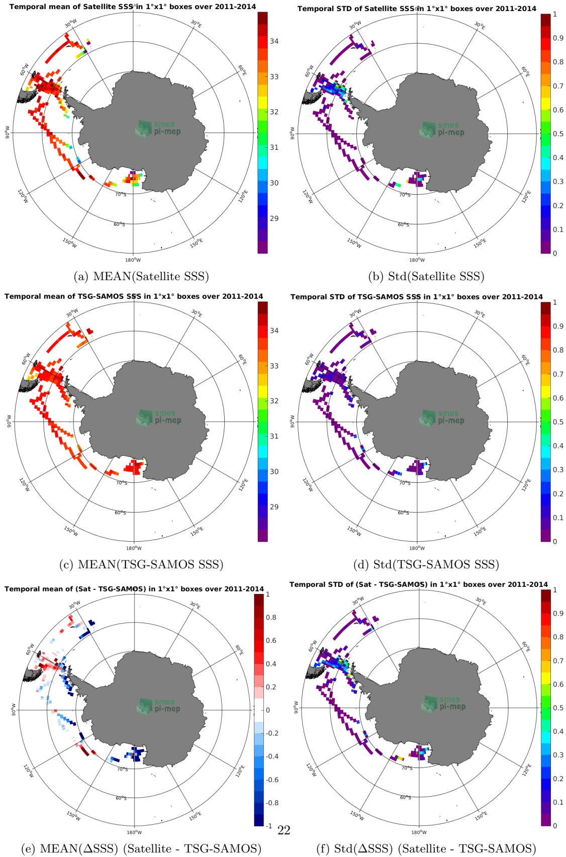
Figure 6: Temporal mean (left) and Std (right) of SSS from Aquarius-L3-OR-V5-MONTHLY-RAIN-MASK-1DEG (top), TSG-SAMOS (middle), and of \Delta SSS (Satellite - TSG-SAMOS). Only match-up pairs are used to generate these maps.
