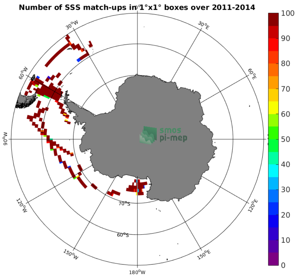
Figure 4: Number of SSS match-ups between TSG-SAMOS SSS and the Aquarius-L3-OR-V5-MONTHLY-RAIN-MASK-1DEG SSS product for the Southern Ocean Pi-MEP region over 1°x1° boxes and for the full satellite product period.
