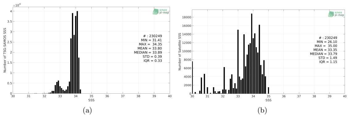
Figure 2: Histograms of SSS from TSG-SAMOS (a) and Aquarius-L3-OR-V5-MONTHLY-RAIN-MASK-1DEG (b) considering all match-up pairs per bins of 0.1 over the Southern Ocean Pi-MEP region and for the full satellite product period.
