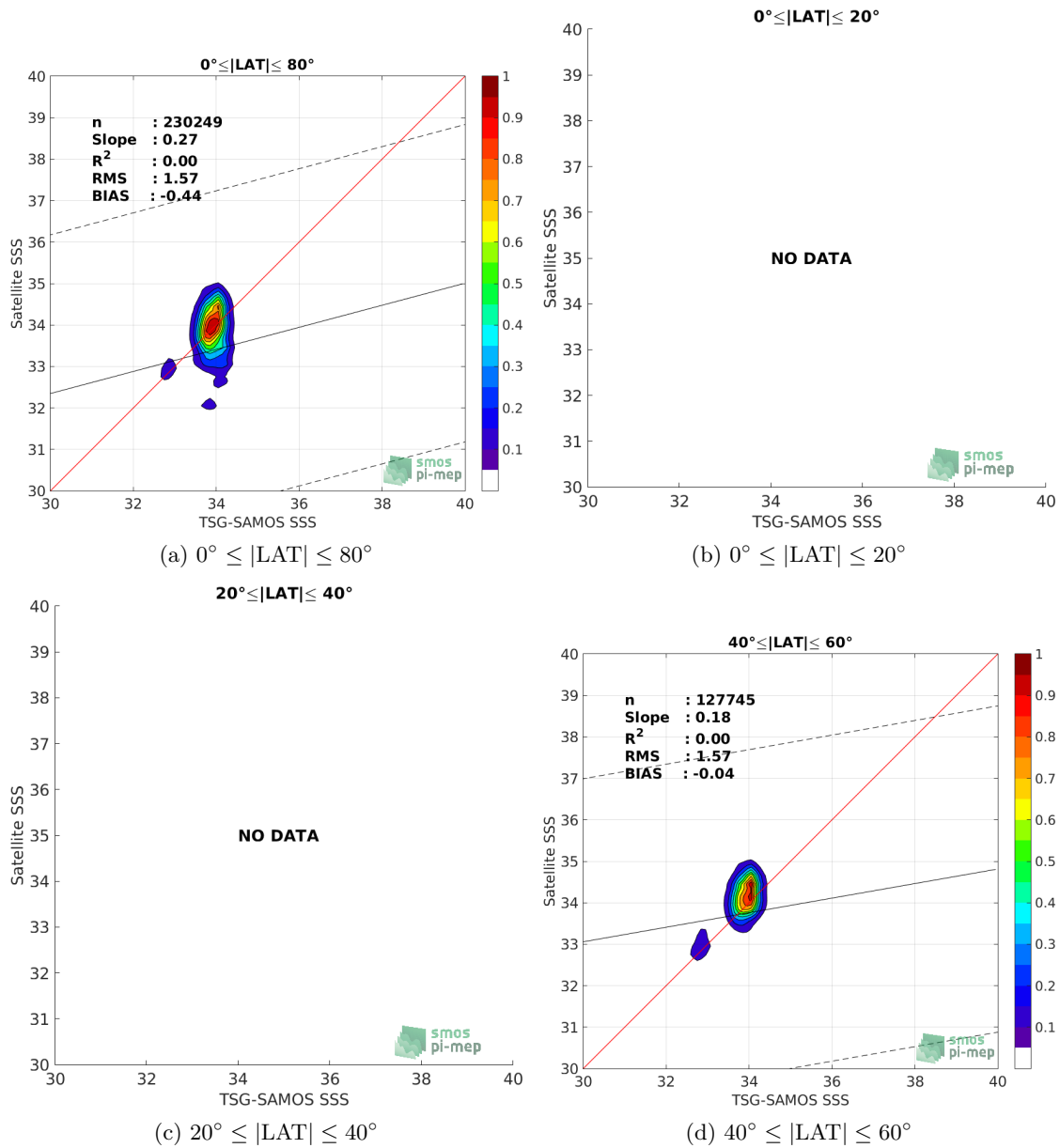
Figure 9: Contour maps of the concentration of Aquarius-L3-OR-V5-MONTHLY-RAIN-MASK-1DEG SSS (y-axis) versus TSG-SAMOS SSS (x-axis) at match-up pairs for different latitude bands. For each plot, the red line shows x=y . The black thin and dashed lines indicate a linear fit through the data cloud and the \pm 95\% confidence levels, respectively. The number match-up pairs n , the slope and R^2 coefficient of the linear fit, the root mean square (RMS) and the mean bias between satellite and in situ data are indicated for each latitude band in each plots.
