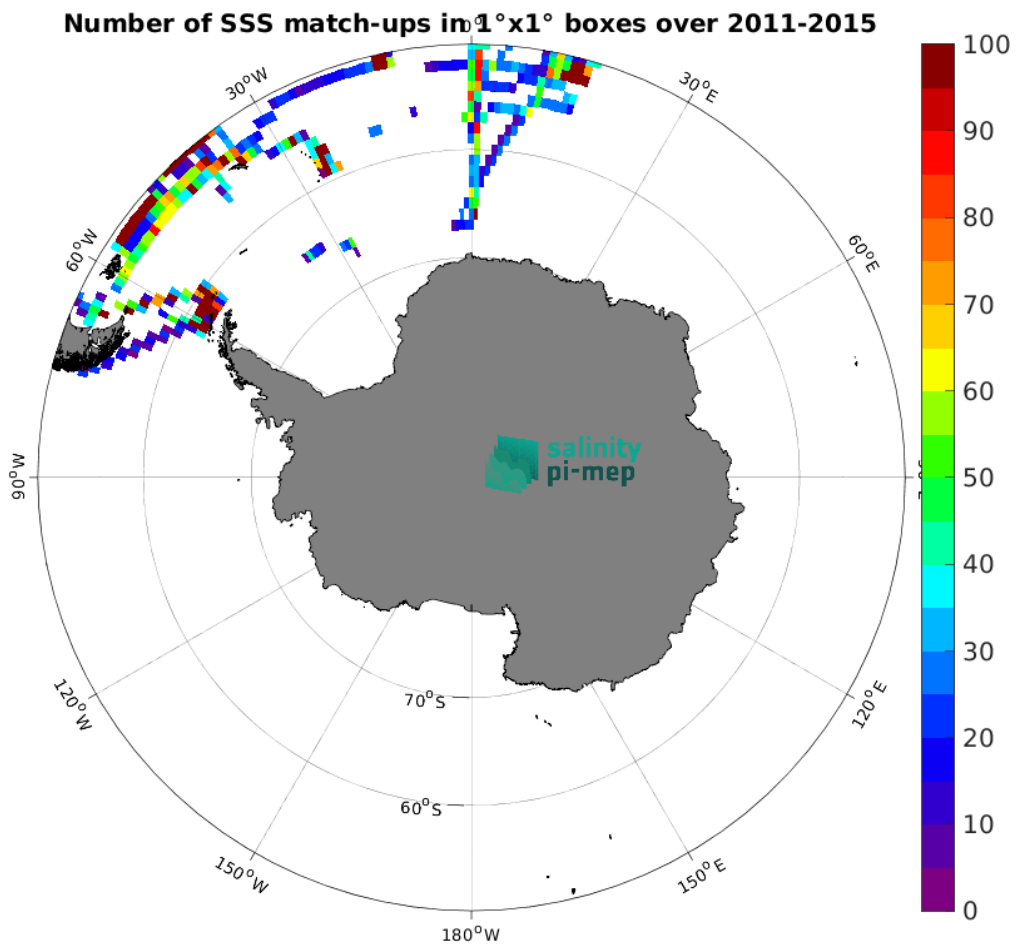
Figure 5: Number of SSS match-ups between TSG (Polarstern) SSS and the Aquarius SSS L3 OR v5 - Monthly - Rain mask (NASA-GSFC) SSS product for the Southern Ocean Pi-MEP region over 1^\circ \times 1^\circ boxes and for the full satellite product period.
