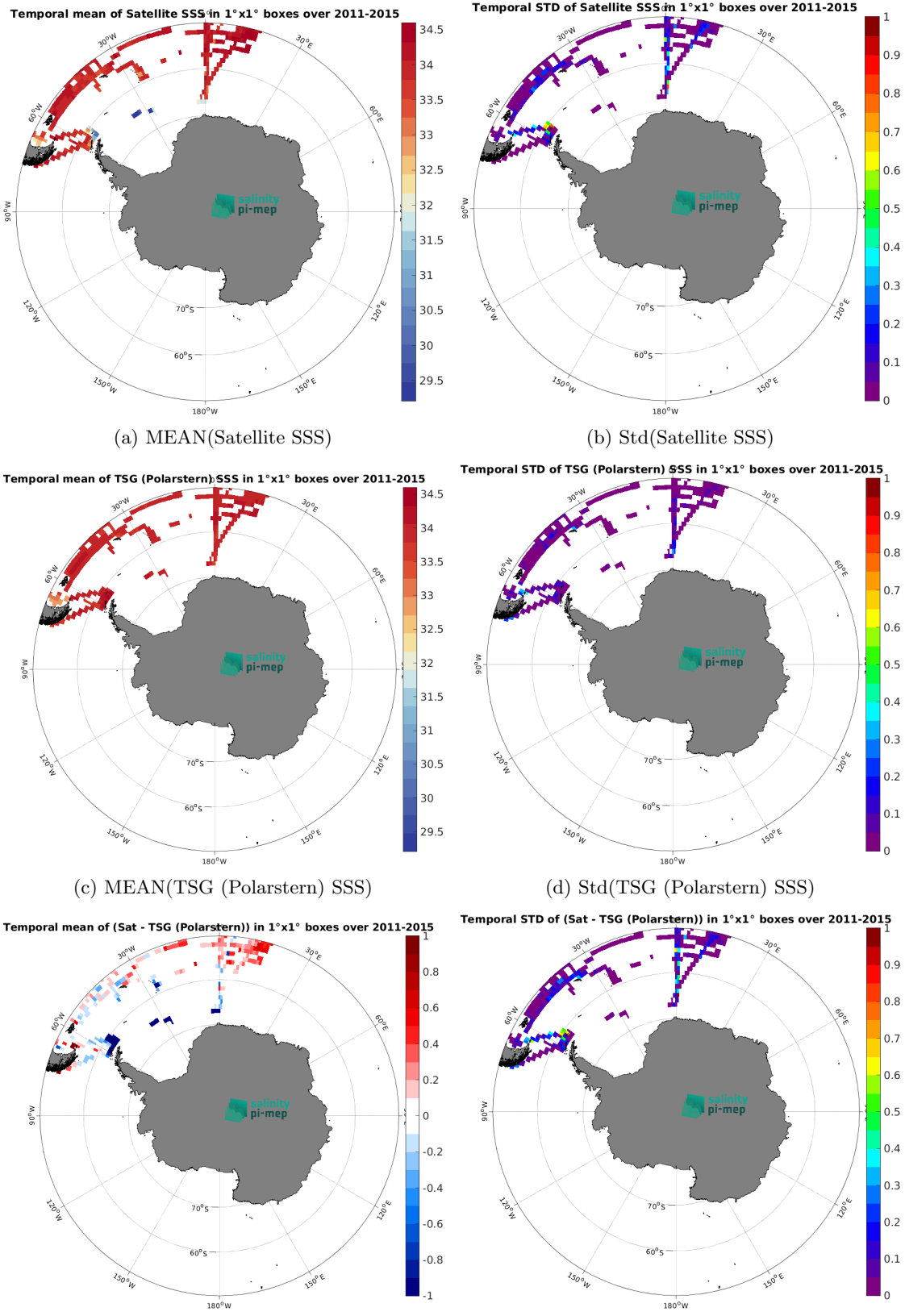
Figure 7: Temporal mean (left) and Std (right) of SSS from Aquarius SSS L3 OR v5 - Monthly - Rain mask (NASA-GSFC) (top), TSG (Polarstern) (middle), and of \Delta SSS (Satellite - TSG (Polarstern)). Only match-up pairs are used to generate these maps.
