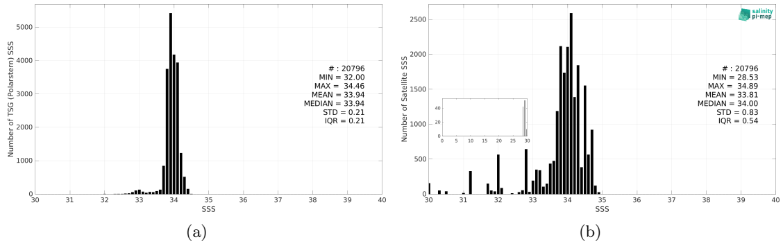
Figure 3: Histograms of SSS from TSG (Polarstern) (a) and Aquarius SSS L3 OR v5 - Monthly - Rain mask (NASA-GSFC) (b) considering all match-up pairs per bins of 0.1 over the Southern Ocean Pi-MEP region and for the full satellite product period.
