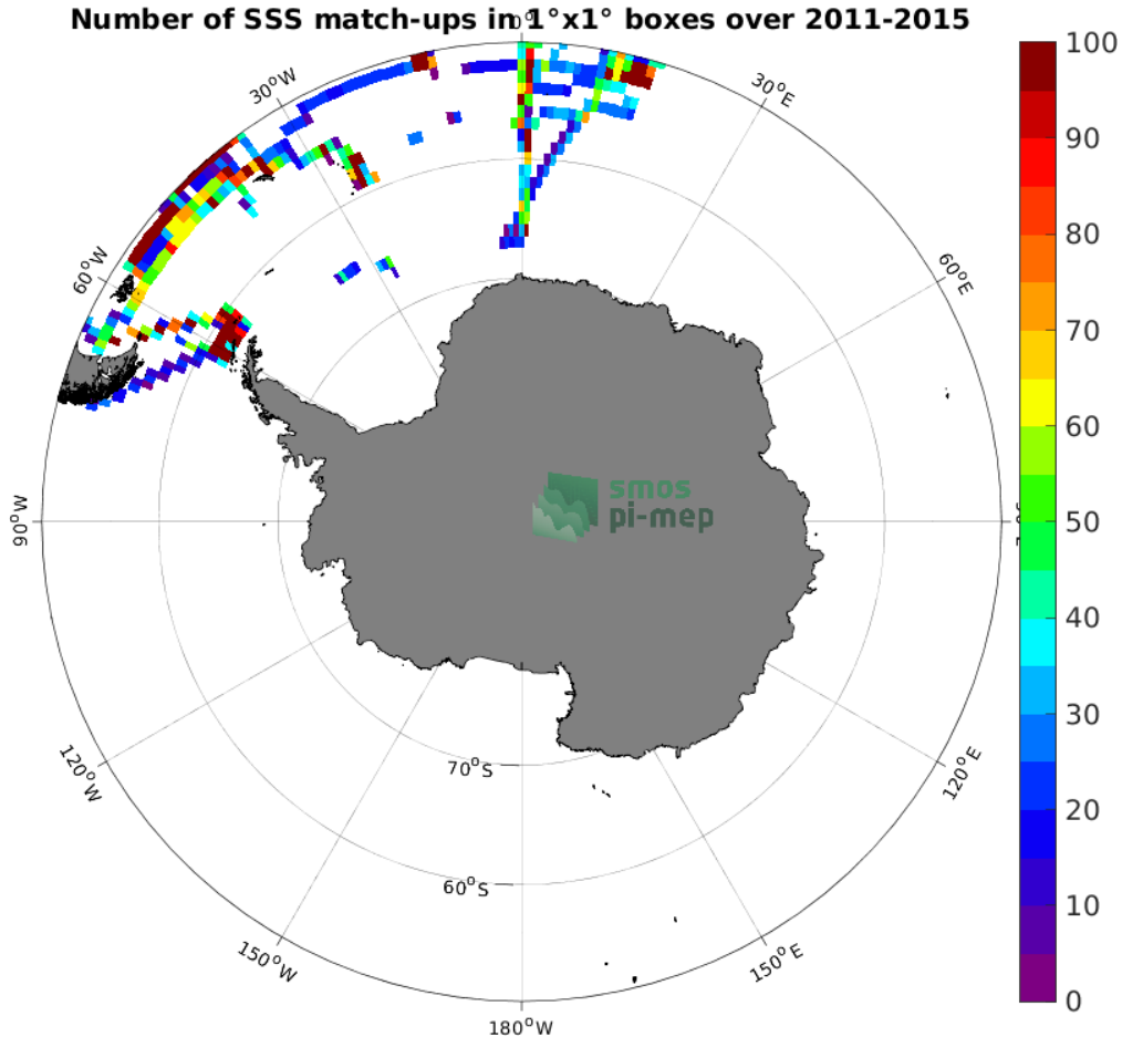
Figure 4: Number of SSS match-ups between TSG (Polarstern) SSS and the Aquarius SSS L3 OR v5 - Monthly - Rain mask (NASA-GSFC) SSS product for the Southern Ocean Pi-MEP region over 1^\circ \times 1^\circ boxes and for the full satellite product period.
