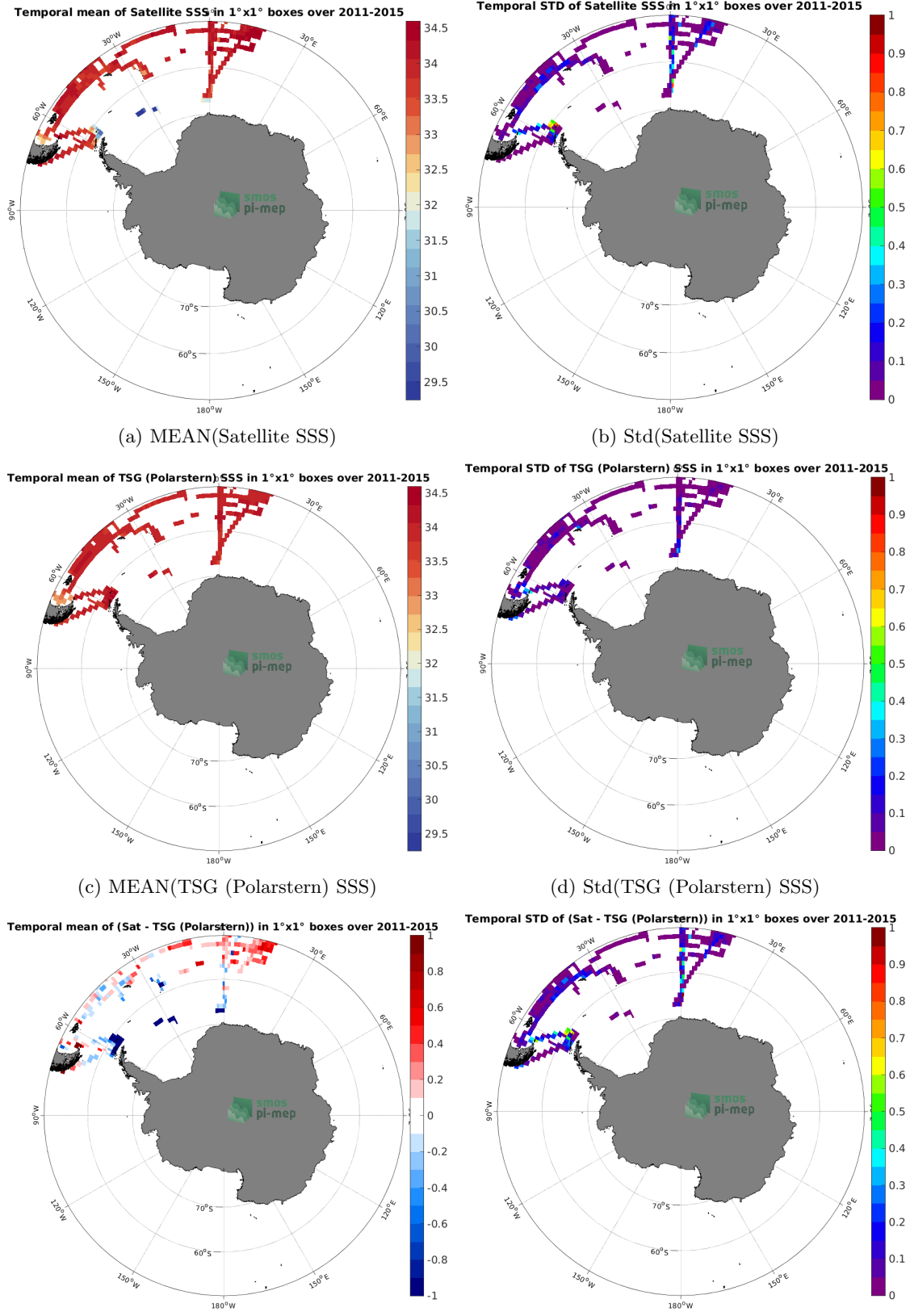
Figure 6: Temporal mean (left) and Std (right) of SSS from Aquarius SSS L3 OR v5 - Monthly - Rain mask (NASA-GSFC) (top), TSG (Polarstern) (middle), and of \Delta SSS (Satellite - TSG (Polarstern)). Only match-up pairs are used to generate these maps.
