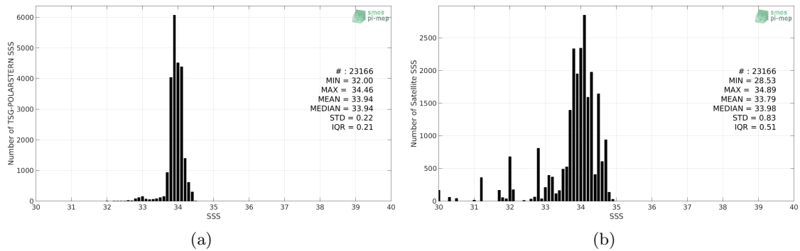
Figure 2: Histograms of SSS from TSG-POLARSTERN (a) and Aquarius-L3-OR-V5-MONTHLY-RAIN-MASK-1DEG (b) considering all match-up pairs per bins of 0.1 over the Southern Ocean Pi-MEP region and for the full satellite product period.
