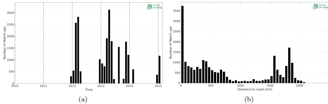
Figure 1: Number of match-ups between TSG-POLARSTERN and Aquarius-L3-OR-V5-MONTHLY-RAIN-MASK-1DEG SSS as a function of time (a) and as function of the distance to coast (b) over the Southern Ocean Pi-MEP region and for the full satellite product period.
