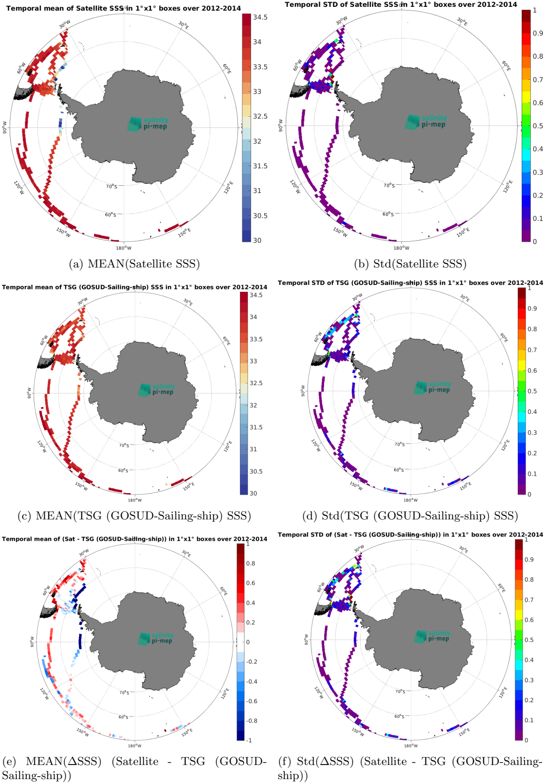
Figure 7: Temporal mean (left) and Std (right), of SSS from Aquarius SSS L3 OR v5 - Monthly - Rain mask (NASA-GSFC) (top), TSG (GOSUD-Sailing-ship) (middle), and of \Delta SSS (Satellite - TSG (GOSUD-Sailing-ship)). Only match-up pairs are used to generate these maps.
