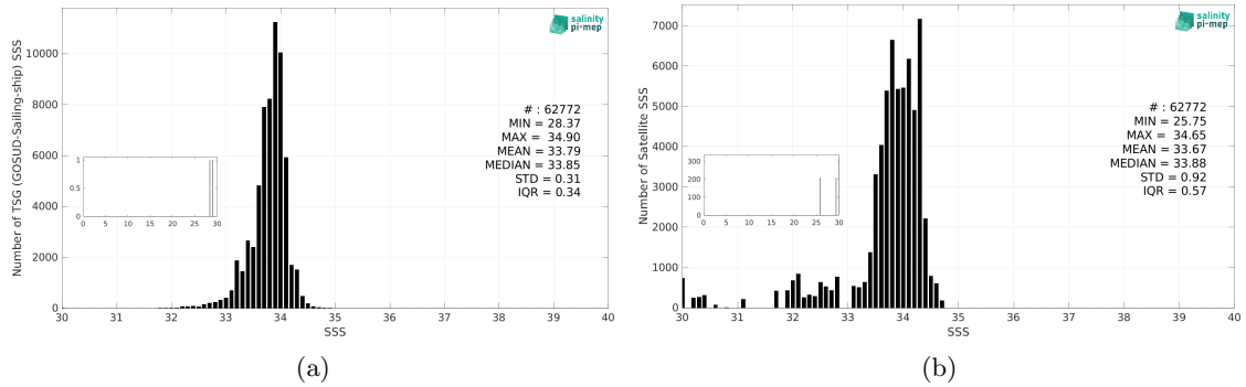
Figure 3: Histograms of SSS from TSG (GOSUD-Sailing-ship) (a) and Aquarius SSS L3 OR v5 - Monthly - Rain mask (NASA-GSFC) (b) considering all match-up pairs per bins of 0.1 over the Southern Ocean Pi-MEP region and for the full satellite product period.
