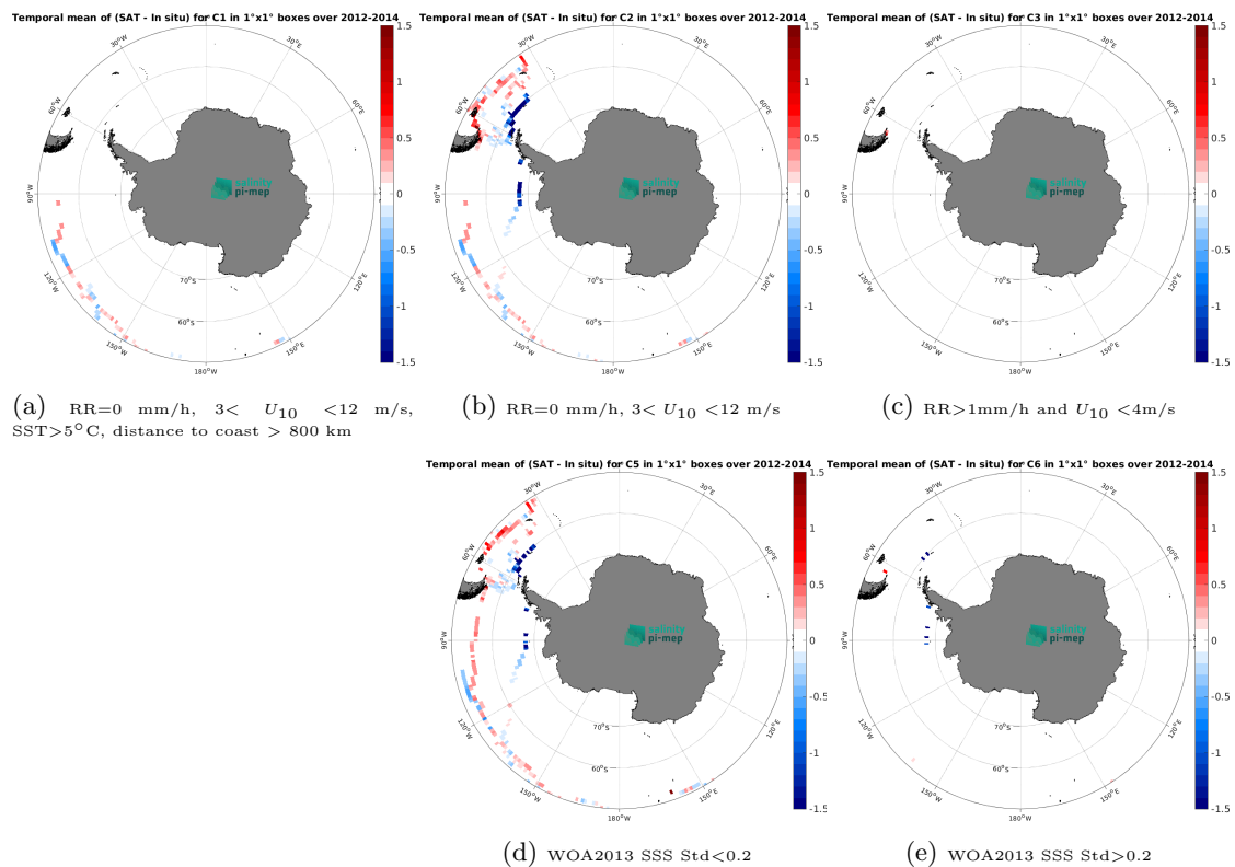
Figure 14: Temporal mean gridded over spatial boxes of size 1^\circ \times 1^\circ of \Delta SSS (Aquarius SSS L3 OR v5 - Monthly - Rain mask (NASA-GSFC) - TSG (GOSUD-Sailing-ship)) for 5 different subdatasets corresponding to:RR=0 mm/h, 3 < U_{10} < 12 m/s, SST > 5^\circ\text{C} , distance to coast > 800 km (a), RR=0 mm/h, 3 < U_{10} < 12 m/s (b), RR > 1 mm/h and U_{10} < 4 m/s (c), WOA2013 SSS Std < 0.2 (d), WOA2013 SSS Std > 0.2 (e).
