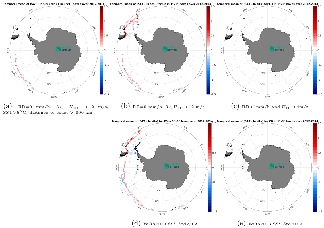
Figure 12: Temporal mean gridded over spatial boxes of size 1^{\circ} \times 1^{\circ} of \Delta\text{SSS} (Aquarius SSS L3 OR v5 - Monthly - Rain mask (NASA-GSFC) - TSG (GOSUD-Sailing-ship)) for 5 different subdatasets corresponding to: RR=0 mm/h, 3 < U_{10} < 12 m/s, SST > 5^{\circ}\text{C} , distance to coast > 800 km (a), RR=0 mm/h, 3 < U_{10} < 12 m/s (b), RR > 1 mm/h and U_{10} < 4 m/s (c), WOA2013 SSS Std < 0.2 (d), WOA2013 SSS Std > 0.2 (e).
