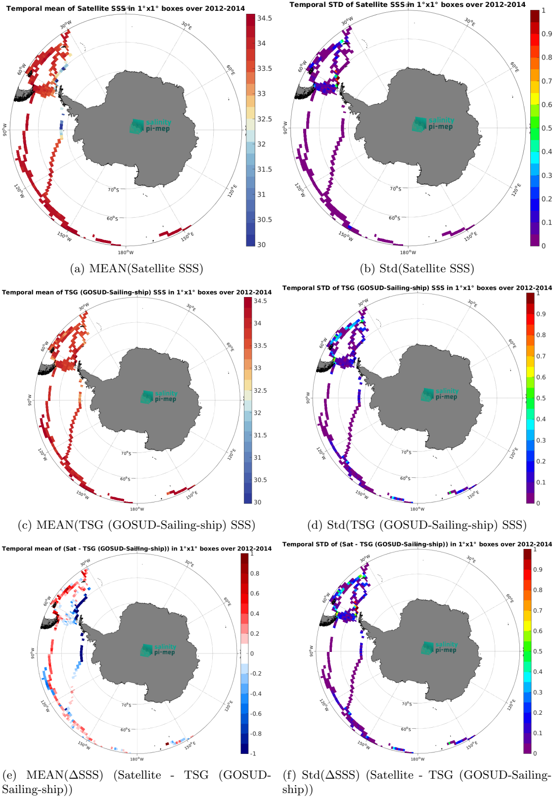
Figure 6: Temporal mean (left) and Std (right) of SSS from Aquarius SSS L3 OR v5 - Monthly - Rain mask (NASA-GSFC) (top), TSG (GOSUD-Sailing-ship) (middle), and of \Delta SSS (Satellite - TSG (GOSUD-Sailing-ship)). Only match-up pairs are used to generate these maps.
