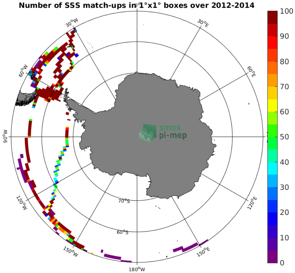
Figure 4: Number of SSS match-ups between TSG (GOSUD-Sailing-ship) SSS and the Aquarius SSS L3 OR v5 - Monthly - Rain mask (NASA-GSFC) SSS product for the Southern Ocean Pi-MEP region over 1^\circ \times 1^\circ boxes and for the full satellite product period.
