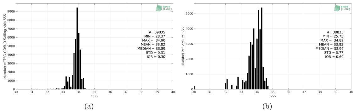
Figure 2: Histograms of SSS from TSG-GOSUD-Sailing-ship (a) and Aquarius-L3-OR-V5-MONTHLY-RAIN-MASK-1DEG (b) considering all match-up pairs per bins of 0.1 over the Southern Ocean Pi-MEP region and for the full satellite product period.
