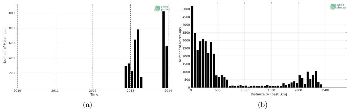
Figure 1: Number of match-ups between TSG-GOSUD-Sailing-ship and Aquarius-L3-OR-V5-MONTHLY-RAIN-MASK-1DEG SSS as a function of time (a) and as function of the distance to coast (b) over the Southern Ocean Pi-MEP region and for the full satellite product period.
