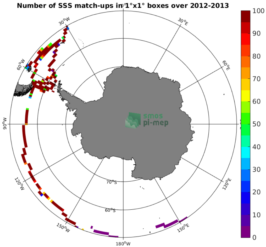
Figure 4: Number of SSS match-ups between TSG-GOSUD-Sailing-ship SSS and the Aquarius-L3-OR-V5-MONTHLY-RAIN-MASK-1DEG SSS product for the Southern Ocean Pi-MEP region over 1^\circ \times 1^\circ boxes and for the full satellite product period.
