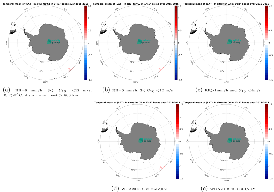
Figure 14: Temporal mean gridded over spatial boxes of size 1^\circ \times 1^\circ of \Delta\text{SSS} (Aquarius SSS L3 OR v5 - Monthly - Rain mask (NASA-GSFC) - TSG (GOSUD-Research-vessel)) for 5 different subdatasets corresponding to:RR=0 mm/h, 3 < U_{10} < 12 m/s, SST>5°C, distance to coast > 800 km (a), RR=0 mm/h, 3 < U_{10} < 12 m/s (b), RR>1mm/h and U_{10} < 4 m/s (c), WOA2013 SSS Std<0.2 (d), WOA2013 SSS Std>0.2 (e).
