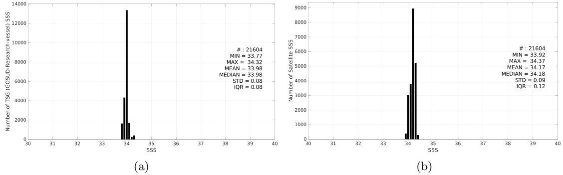
Figure 3: Histograms of SSS from TSG (GOSUD-Research-vessel) (a) and Aquarius SSS L3 OR v5 - Monthly - Rain mask (NASA-GSFC) (b) considering all match-up pairs per bins of 0.1 over the Southern Ocean Pi-MEP region and for the full satellite product period.
