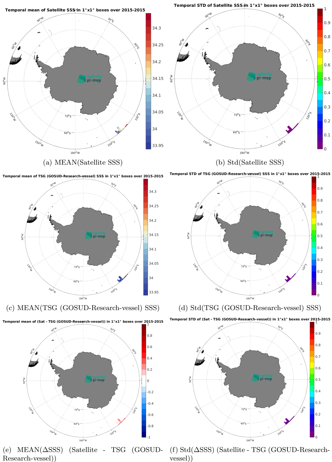
Figure 7: Temporal mean (left) and Std (right) of SSS from Aquarius SSS L3 OR v5 - Monthly - Rain mask (NASA-GSFC) (top), TSG (GOSUD-Research-vessel) (middle), and of \Delta SSS (Satellite - TSG (GOSUD-Research-vessel)). Only 16 up-ch pairs are used to generate these maps.
