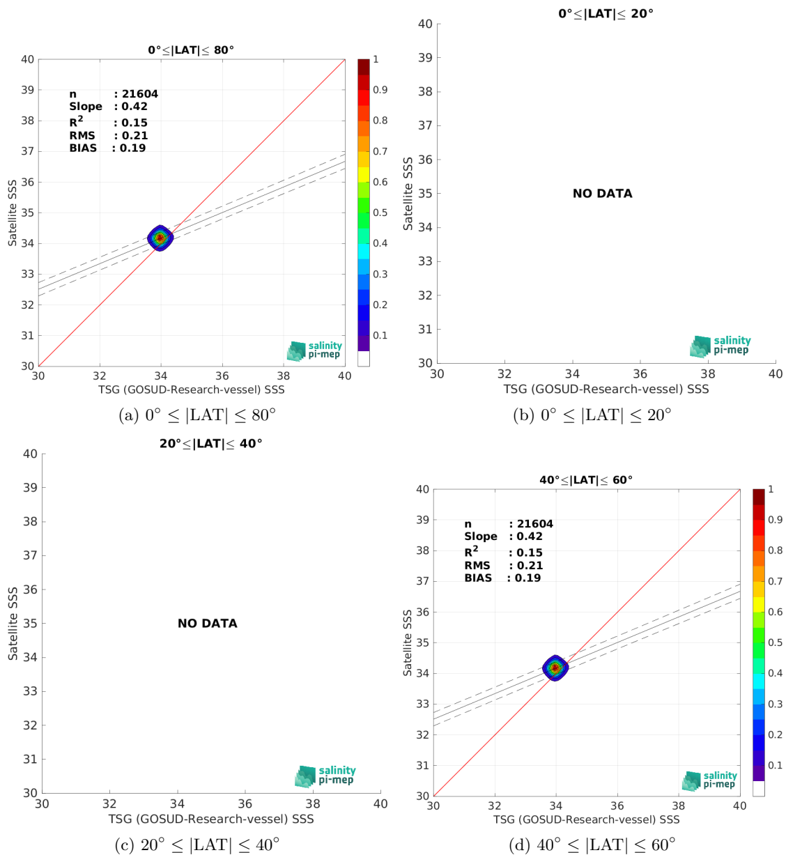
Figure 10: Contour maps of the concentration of Aquarius SSS L3 OR v5 - Monthly - Rain mask (NASA-GSFC) SSS (y-axis) versus TSG (GOSUD-Research-vessel) SSS (x-axis) at match-up pairs for different latitude bands. For each plot, the red line shows x=y . The black thin and dashed lines indicate a linear fit through the data cloud and the \pm 95\% confidence levels, respectively. The number match-up pairs n , the slope and R^2 coefficient of the linear fit, the root mean square (RMS) and the mean bias between satellite and in situ data are indicated for each latitude band in each plots.
