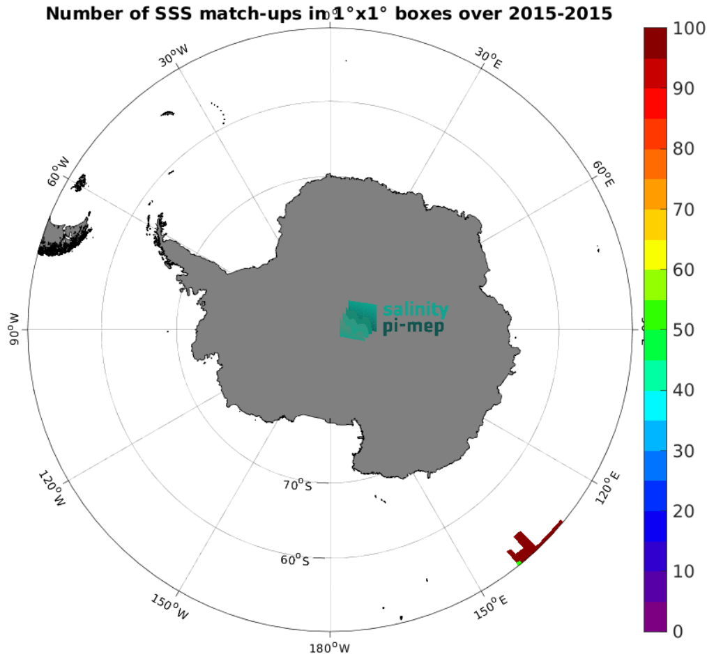
Figure 5: Number of SSS match-ups between TSG (GOSUD-Research-vessel) SSS and the Aquarius SSS L3 OR v5 - Monthly - Rain mask (NASA-GSFC) SSS product for the Southern Ocean Pi-MEP region over 1^\circ \times 1^\circ boxes and for the full satellite product period.
