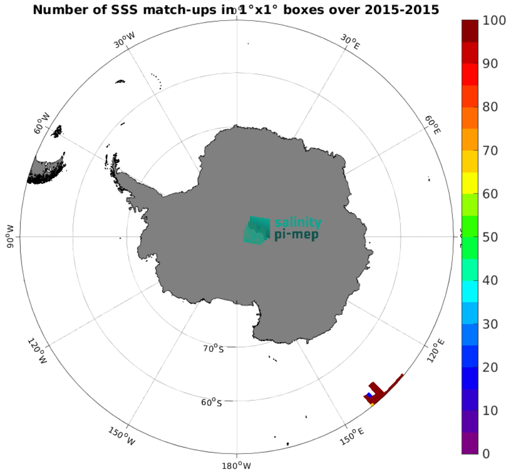
Figure 4: Number of SSS match-ups between TSG (GOSUD-Research-vessel) SSS and the Aquarius SSS L3 OR v5 - Monthly - Rain mask (NASA-GSFC) SSS product for the Southern Ocean Pi-MEP region over 1^\circ \times 1^\circ boxes and for the full satellite product period.
