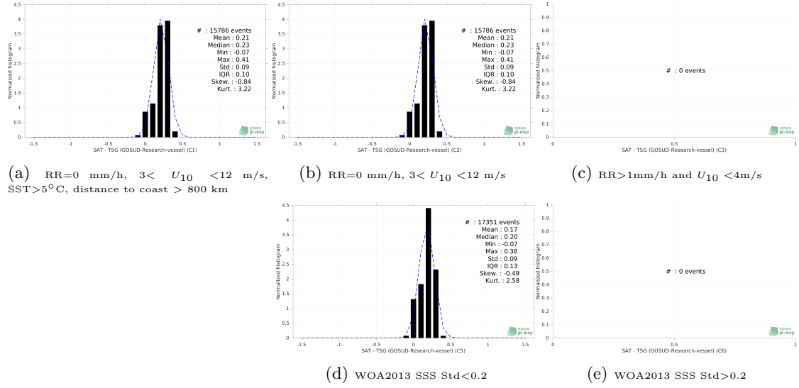
Figure 13: Normalized histogram of \Delta\text{SSS} (Aquarius SSS L3 OR v5 - Monthly - Rain mask (NASA-GSFC) - TSG (GOSUD-Research-vessel)) for 5 different subdatasets corresponding to: RR=0 mm/h, 3 < U_{10} < 12 m/s, SST > 5^\circ\text{C} , distance to coast > 800 km (a), RR=0 mm/h, 3 < U_{10} < 12 m/s (b), RR > 1\text{mm/h} and U_{10} < 4\text{m/s} (c), WOA2013 SSS \text{Std} < 0.2 (d), WOA2013 SSS \text{Std} > 0.2 (e).
