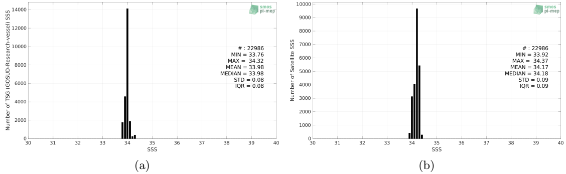
Figure 2: Histograms of SSS from TSG (GOSUD-Research-vessel) (a) and Aquarius SSS L3 OR v5 - Monthly - Rain mask (NASA-GSFC) (b) considering all match-up pairs per bins of 0.1 over the Southern Ocean Pi-MEP region and for the full satellite product period.
