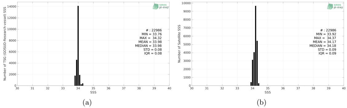
Figure 2: Histograms of SSS from TSG (GOSUD-Research-vessel) (a) and Aquarius SSS L3 OR v5 - Monthly - Rain mask (NASA-GSFC) (b) considering all match-up pairs per bins of 0.1 over the Southern Ocean Pi-MEP region and for the full satellite product period.
