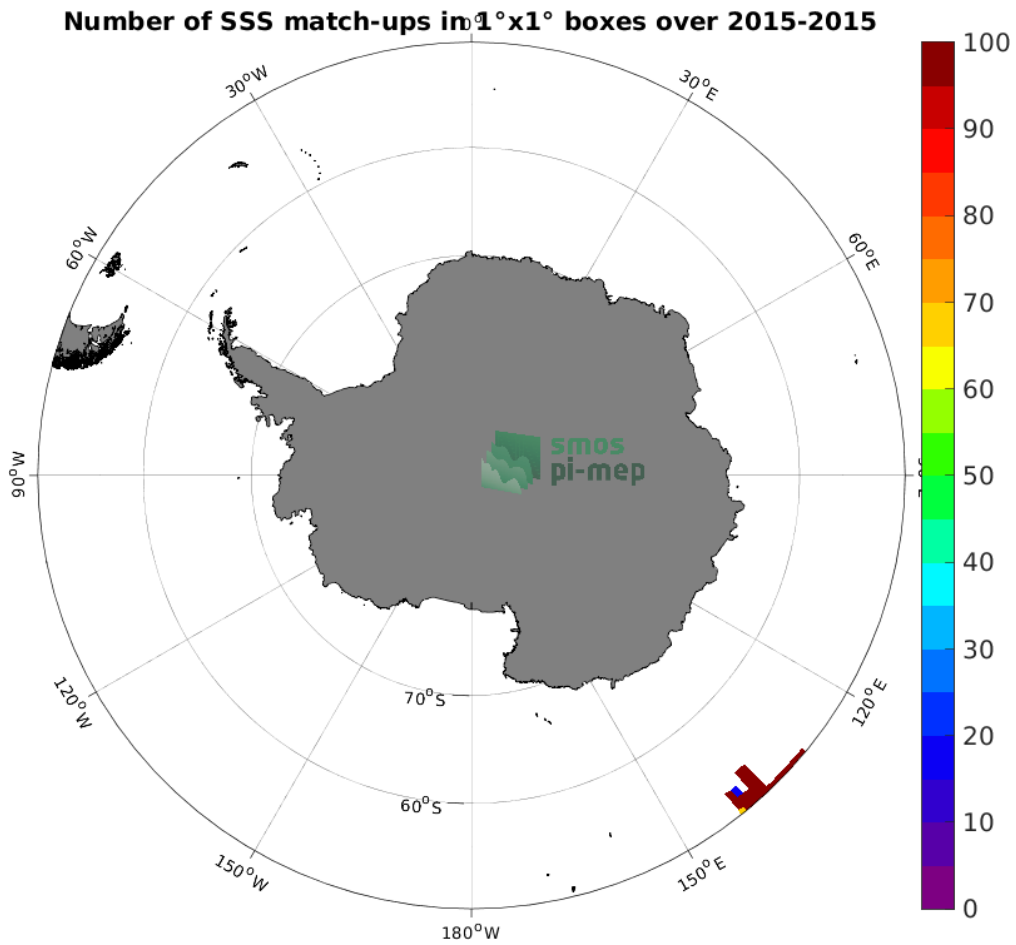
Figure 4: Number of SSS match-ups between TSG (GOSUD-Research-vessel) SSS and the Aquarius SSS L3 OR v5 - Monthly - Rain mask (NASA-GSFC) SSS product for the Southern Ocean Pi-MEP region over 1^\circ \times 1^\circ boxes and for the full satellite product period.
