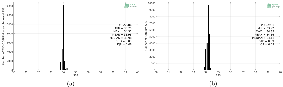
Figure 2: Histograms of SSS from TSG-GOSUD-Research-vessel (a) and Aquarius-L3-OR-V5-MONTHLY-RAIN-MASK-1DEG (b) considering all match-up pairs per bins of 0.1 over the Southern Ocean Pi-MEP region and for the full satellite product period.
