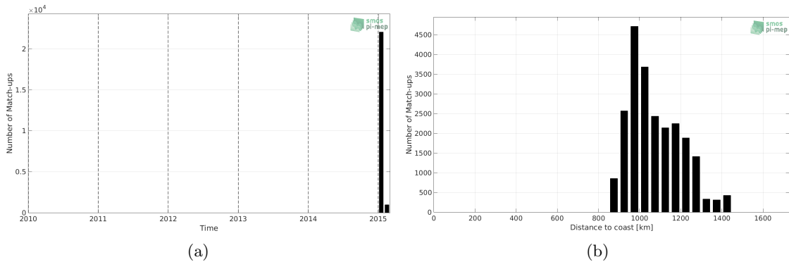
Figure 1: Number of match-ups between TSG-GOSUD-Research-vessel and Aquarius-L3-OR-V5-MONTHLY-RAIN-MASK-1DEG SSS as a function of time (a) and as function of the distance to coast (b) over the Southern Ocean Pi-MEP region and for the full satellite product period.
