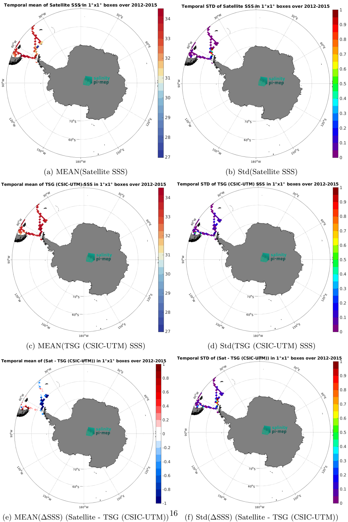
Figure 7: Temporal mean (left) and Std (right) of SSS from Aquarius SSS L3 OR v5 - Monthly - Rain mask (NASA-GSFC) (top), TSG (CSIC-UTM) (middle), and of \Delta SSS (Satellite - TSG (CSIC-UTM)). Only match-up pairs are used to generate these maps.
