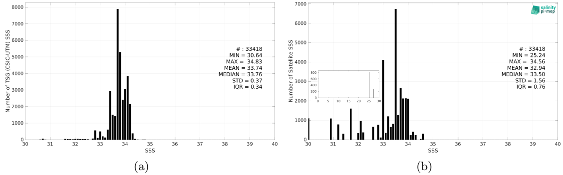
Figure 3: Histograms of SSS from TSG (CSIC-UTM) (a) and Aquarius SSS L3 OR v5 - Monthly - Rain mask (NASA-GSFC) (b) considering all match-up pairs per bins of 0.1 over the Southern Ocean Pi-MEP region and for the full satellite product period.
