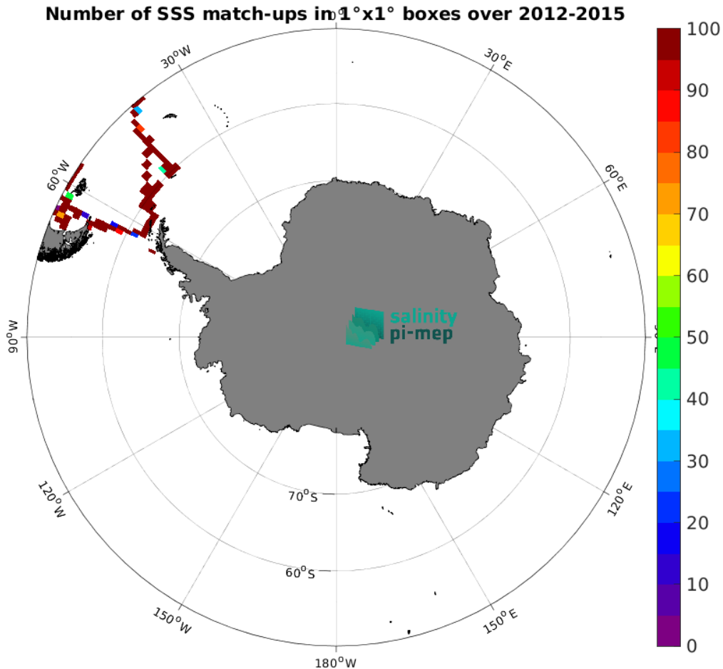
Figure 5: Number of SSS match-ups between TSG (CSIC-UTM) SSS and the Aquarius SSS L3 OR v5 - Monthly - Rain mask (NASA-GSFC) SSS product for the Southern Ocean Pi-MEP region over 1^\circ \times 1^\circ boxes and for the full satellite product period.
