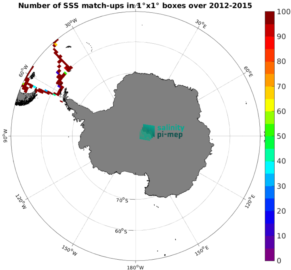
Figure 4: Number of SSS match-ups between TSG (CSIC-UTM) SSS and the Aquarius SSS L3 OR v5 - Monthly - Rain mask (NASA-GSFC) SSS product for the Southern Ocean Pi-MEP region over 1^\circ \times 1^\circ boxes and for the full satellite product period.
