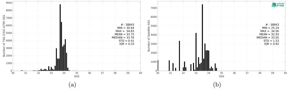
Figure 2: Histograms of SSS from TSG (CSIC-UTM) (a) and Aquarius SSS L3 OR v5 - Monthly - Rain mask (NASA-GSFC) (b) considering all match-up pairs per bins of 0.1 over the Southern Ocean Pi-MEP region and for the full satellite product period.
