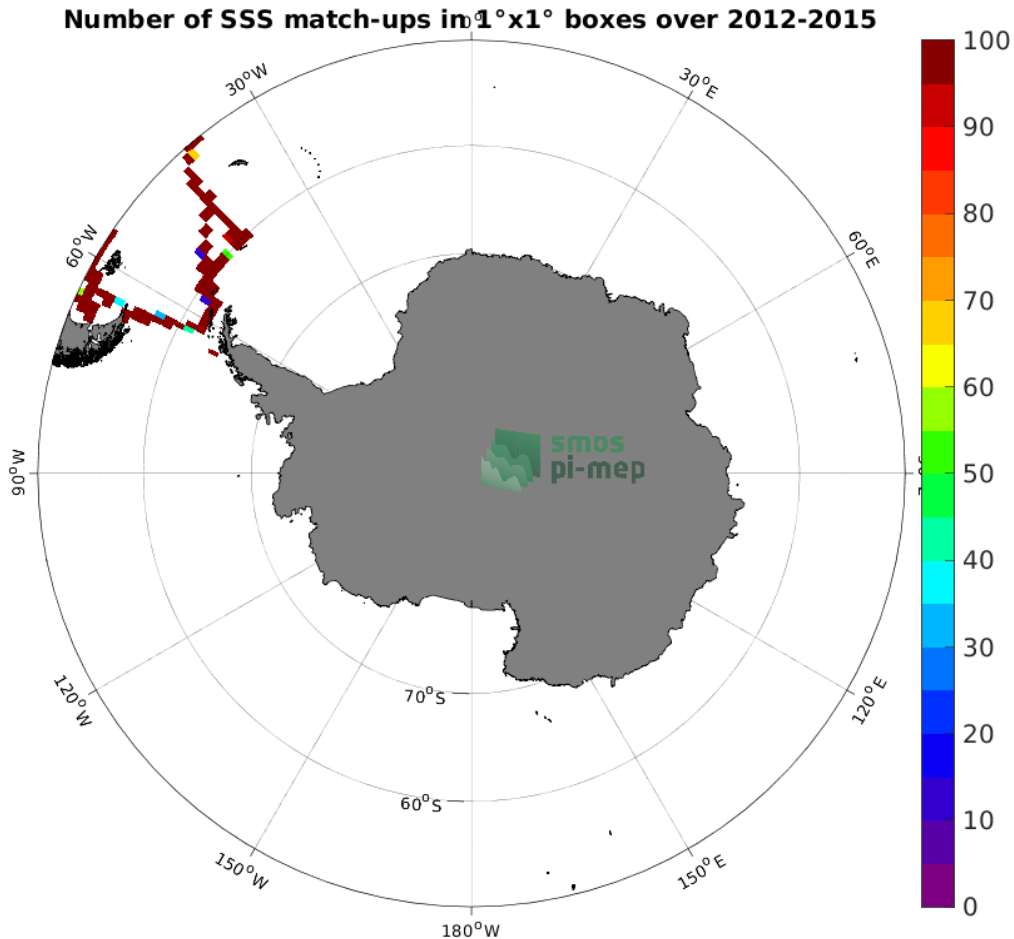
Figure 4: Number of SSS match-ups between TSG (CSIC-UTM) SSS and the Aquarius SSS L3 OR v5 - Monthly - Rain mask (NASA-GSFC) SSS product for the Southern Ocean Pi-MEP region over 1^\circ \times 1^\circ boxes and for the full satellite product period.
