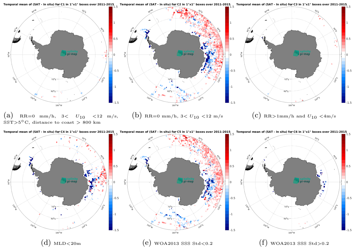
Figure 14: Temporal mean gridded over spatial boxes of size 1^\circ \times 1^\circ of \Delta\text{SSS} (Aquarius SSS L3 OR v5 - Monthly - Rain mask (NASA-GSFC) - Marine mammals) for 6 different subdatasets corresponding to:RR=0 mm/h, 3 < U_{10} < 12 m/s, SST>5°C, distance to coast > 800 km (a), RR=0 mm/h, 3 < U_{10} < 12 m/s (b), RR>1mm/h and U_{10} < 4 m/s (c),MLD<20m (d),WOA2013 SSS Std<0.2 (e),WOA2013 SSS Std>0.2 (f).
