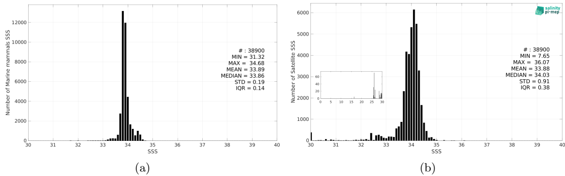
Figure 3: Histograms of SSS from Marine mammals (a) and Aquarius SSS L3 OR v5 - Monthly - Rain mask (NASA-GSFC) (b) considering all match-up pairs per bins of 0.1 over the Southern Ocean Pi-MEP region and for the full satellite product period.
