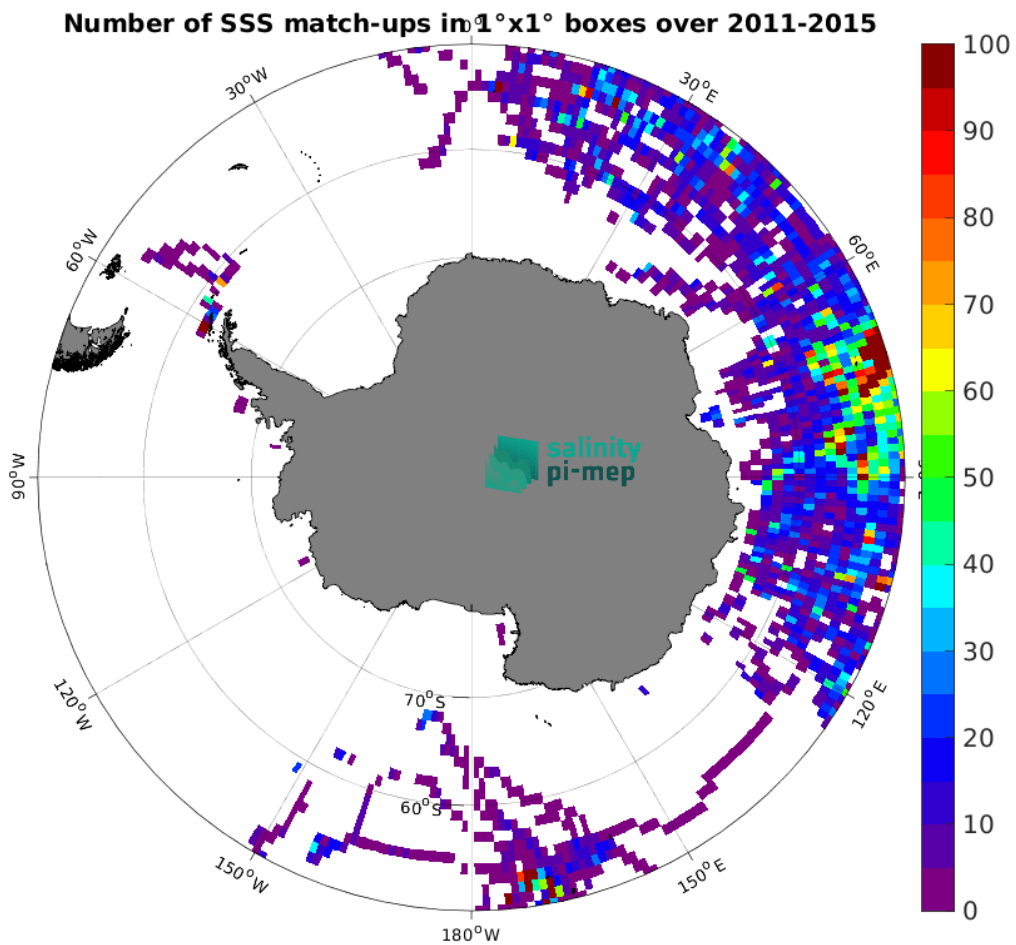
Figure 5: Number of SSS match-ups between Marine mammals SSS and the Aquarius SSS L3 OR v5 - Monthly - Rain mask (NASA-GSFC) SSS product for the Southern Ocean Pi-MEP region over 1^\circ \times 1^\circ boxes and for the full satellite product period.
