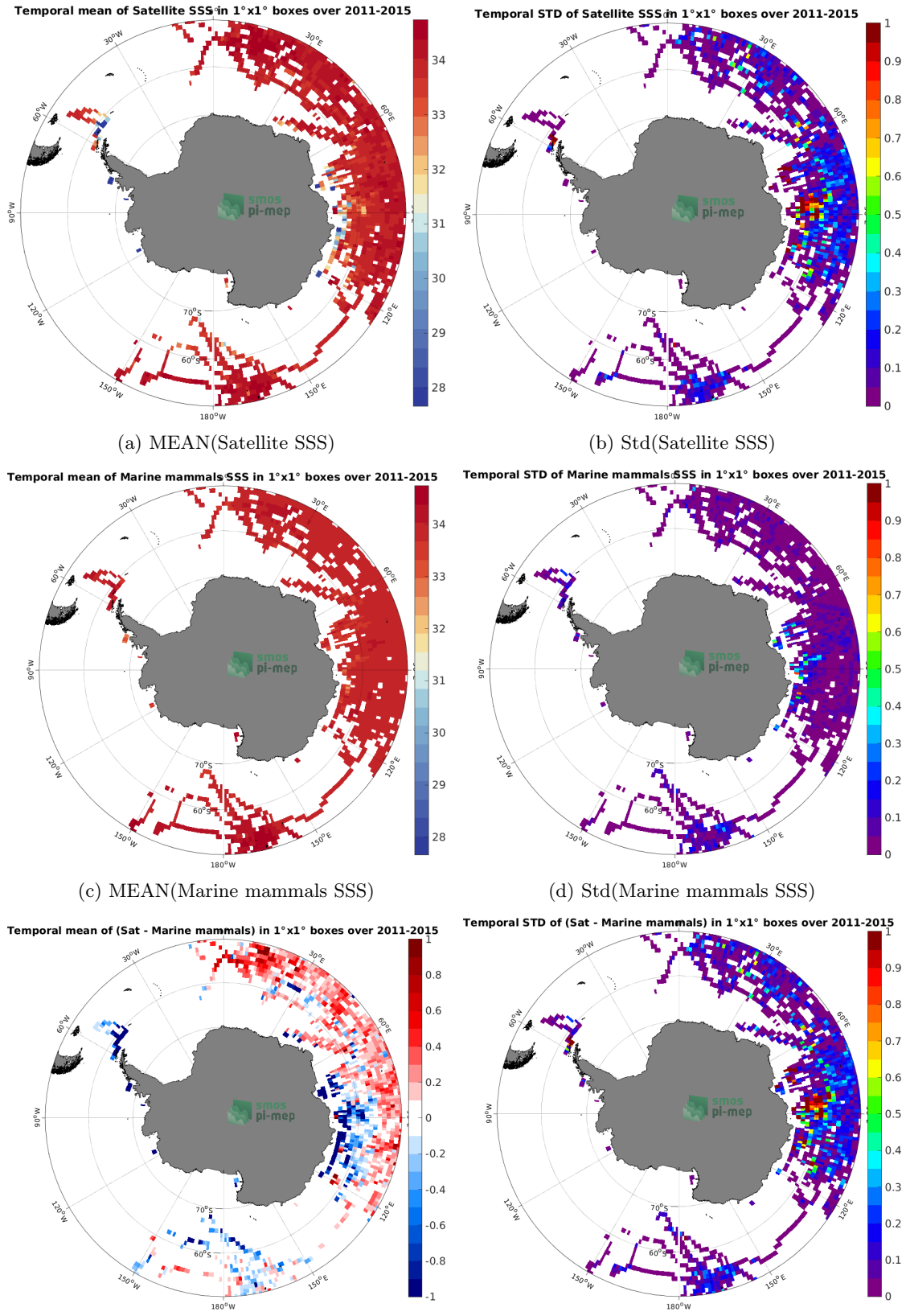
Figure 6: Temporal mean (left) and Std (right) of SSS from Aquarius SSS L3 OR v5 - Monthly - Rain mask (NASA-GSFC) (top), Marine mammals (middle), and of \Delta SSS (Satellite - Marine mammals). Only match-up pairs are used to generate these maps.
