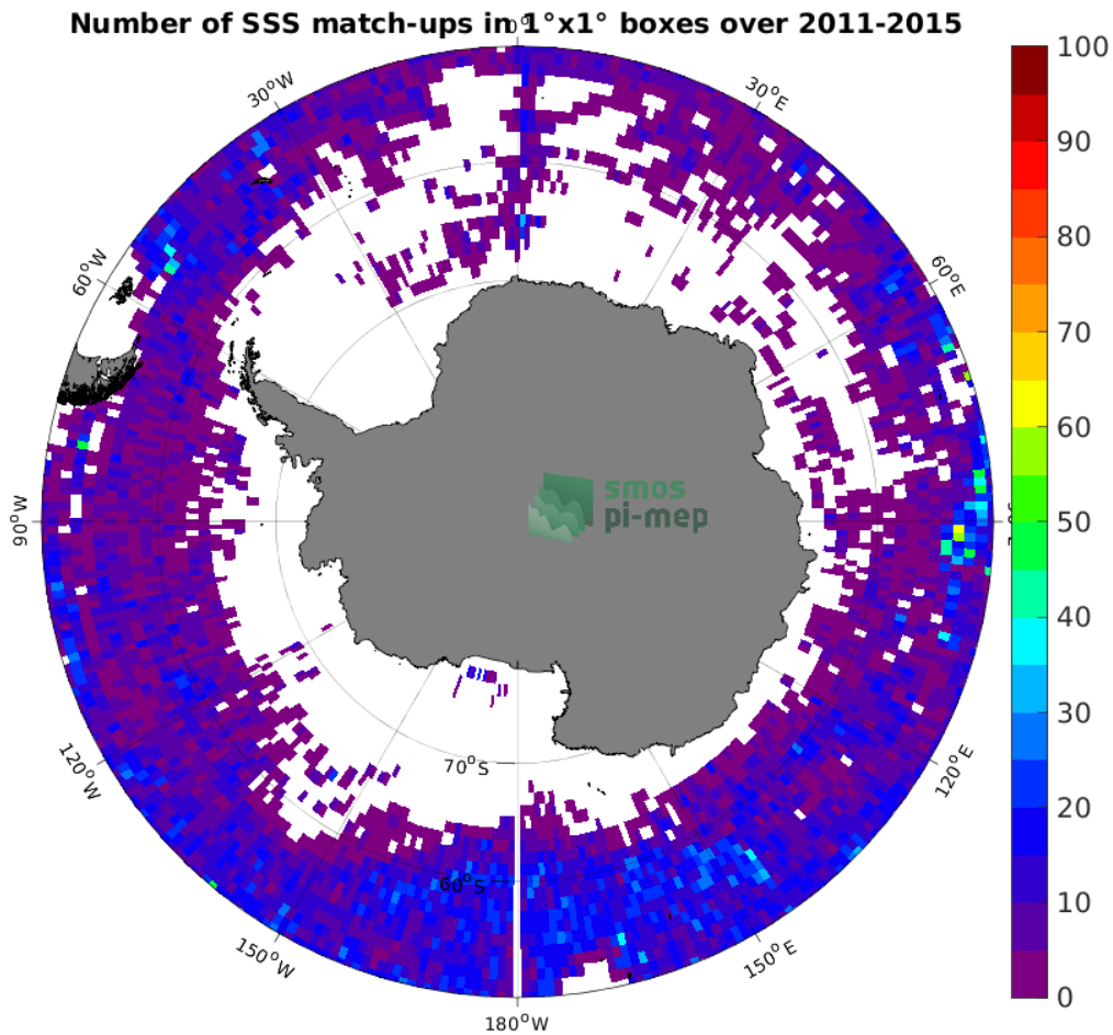
Figure 4: Number of SSS match-ups between Argo SSS and the Aquarius SSS L3 OR v5 - Monthly - Rain mask (NASA-GSFC) SSS product for the Southern Ocean Pi-MEP region over 1^\circ \times 1^\circ boxes and for the full satellite product period.
