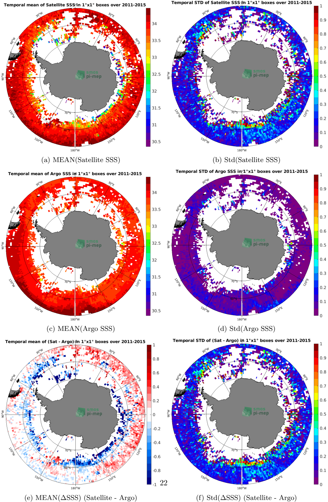
Figure 6: Temporal mean (left) and Std (right) of SSS from Aquarius SSS L3 OR v5 - Monthly - Rain mask (NASA-GSFC) (top), Argo (middle), and of \Delta SSS (Satellite - Argo). Only match-up pairs are used to generate these maps.
