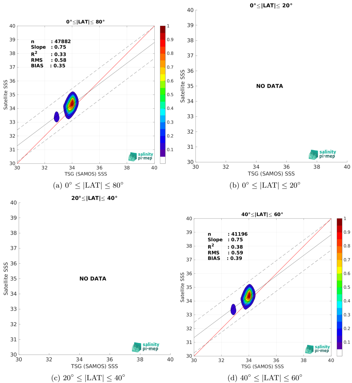
Figure 10: Contour maps of the concentration of Aquarius SSS L3 CAP v5 - 7-Day running (JPL) SSS (y-axis) versus TSG (SAMOS) SSS (x-axis) at match-up pairs for different latitude bands. For each plot, the red line shows x=y . The black thin and dashed lines indicate a linear fit through the data cloud and the \pm 95\% confidence levels, respectively. The number match-up pairs n , the slope and R^2 coefficient of the linear fit, the root mean square (RMS) and the mean bias between satellite and in situ data are indicated for each latitude band in each plots.
