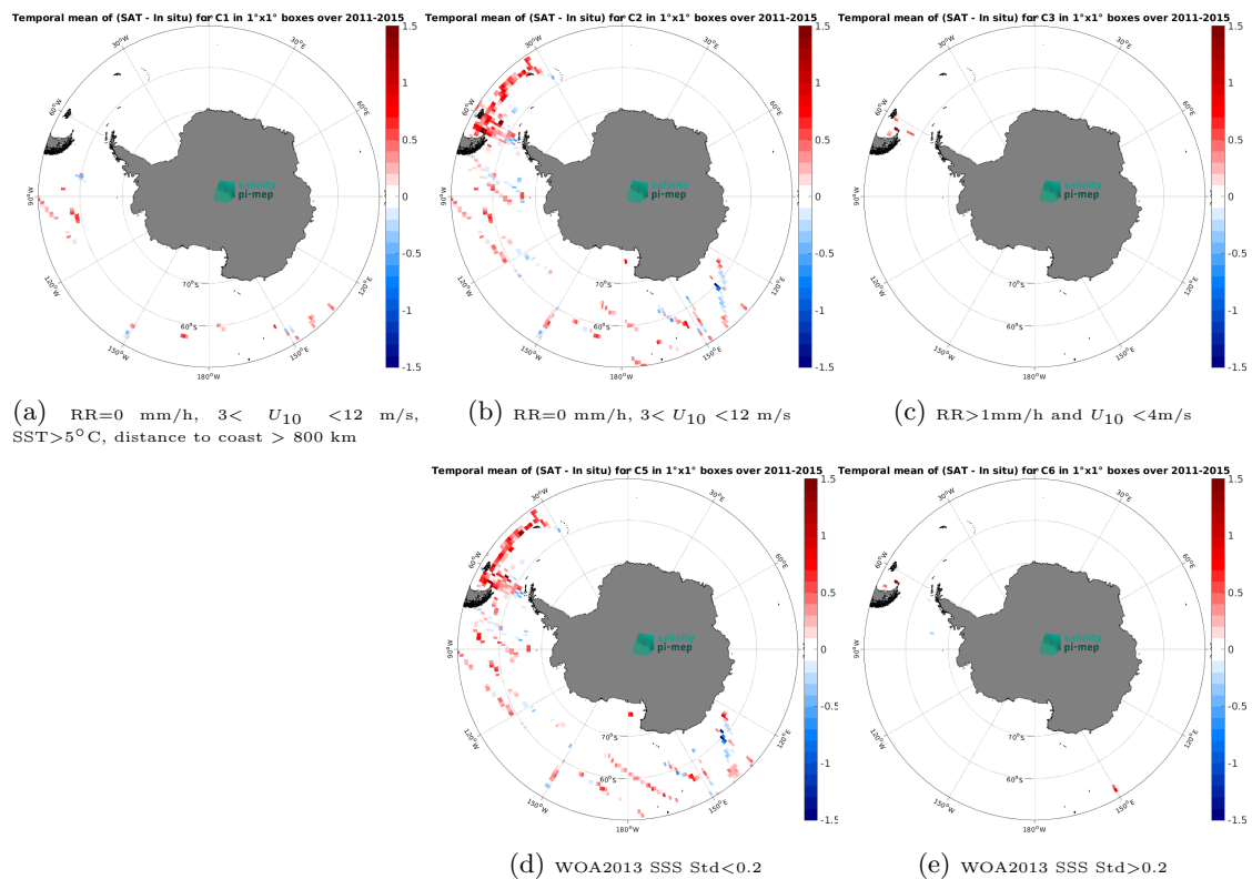
Figure 14: Temporal mean gridded over spatial boxes of size 1^\circ \times 1^\circ of \Delta\text{SSS} (Aquarius SSS L3 CAP v5 - 7-Day running (JPL) - TSG (SAMOS)) for 5 different subdatasets corresponding to:RR=0 mm/h, 3 < U_{10} < 12 m/s, SST>5°C, distance to coast > 800 km (a), RR=0 mm/h, 3 < U_{10} < 12 m/s (b), RR>1mm/h and U_{10} < 4 m/s (c), WOA2013 SSS Std<0.2 (d), WOA2013 SSS Std>0.2 (e).
