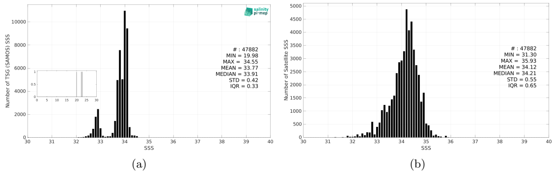
Figure 3: Histograms of SSS from TSG (SAMOS) (a) and Aquarius SSS L3 CAP v5 - 7-Day running (JPL) (b) considering all match-up pairs per bins of 0.1 over the Southern Ocean Pi-MEP region and for the full satellite product period.
