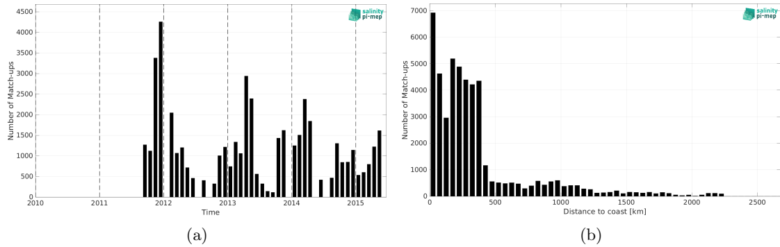
Figure 2: Number of match-ups between TSG (SAMOS) and Aquarius SSS L3 CAP v5 - 7-Day running (JPL) SSS as a function of time (a) and as function of the distance to coast (b) over the Southern Ocean Pi-MEP region and for the full satellite product period.
