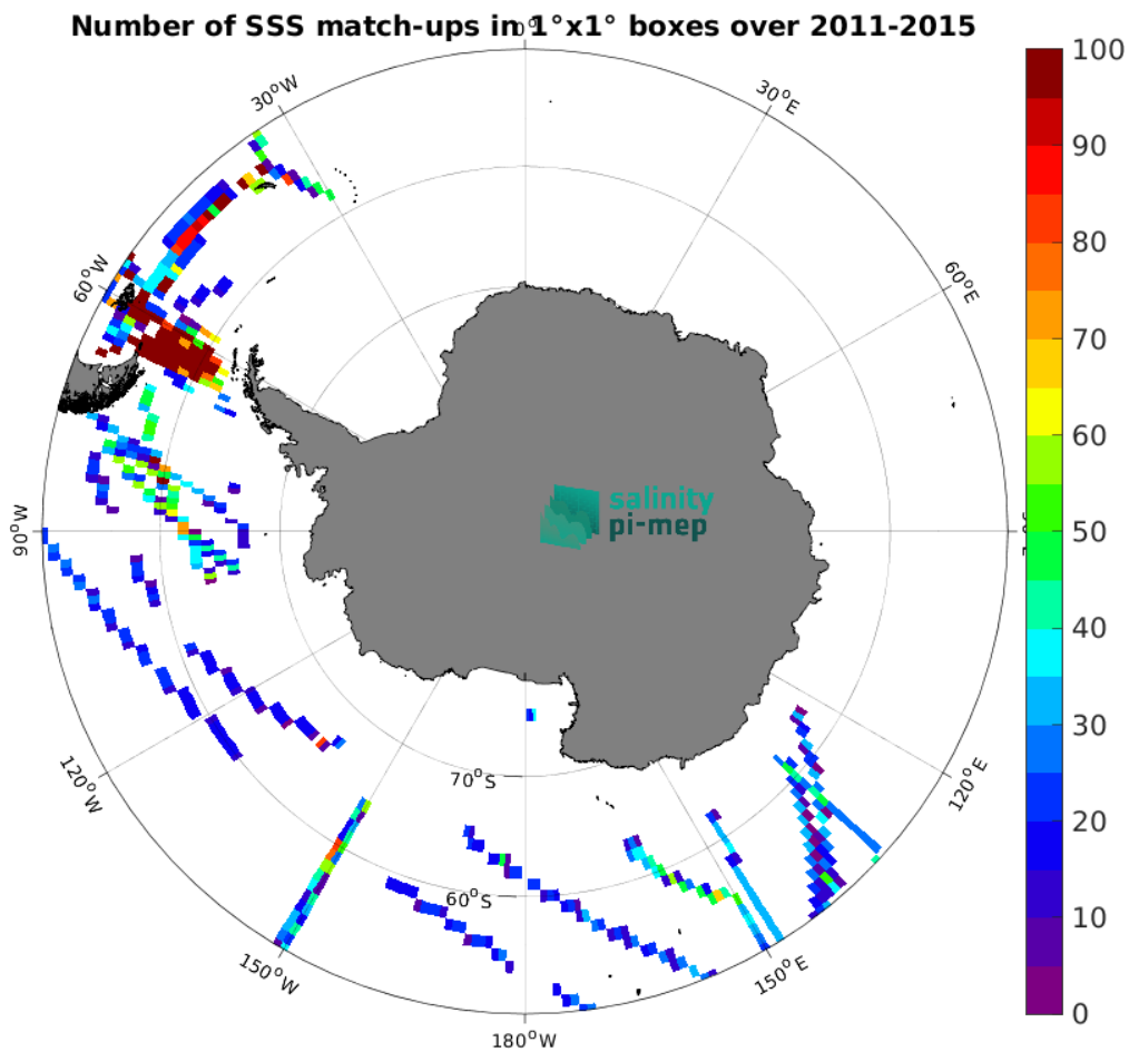
Figure 5: Number of SSS match-ups between TSG (SAMOS) SSS and the Aquarius SSS L3 CAP v5 - 7-Day running (JPL) SSS product for the Southern Ocean Pi-MEP region over 1^{\circ} \times 1^{\circ} boxes and for the full satellite product period.
