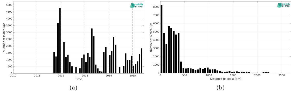
Figure 1: Number of match-ups between TSG (SAMOS) and Aquarius SSS L3 CAP v5 - 7-Day running (JPL) SSS as a function of time (a) and as function of the distance to coast (b) over the Southern Ocean Pi-MEP region and for the full satellite product period.
