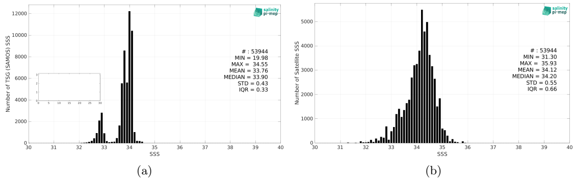
Figure 2: Histograms of SSS from TSG (SAMOS) (a) and Aquarius SSS L3 CAP v5 - 7-Day running (JPL) (b) considering all match-up pairs per bins of 0.1 over the Southern Ocean Pi-MEP region and for the full satellite product period.
