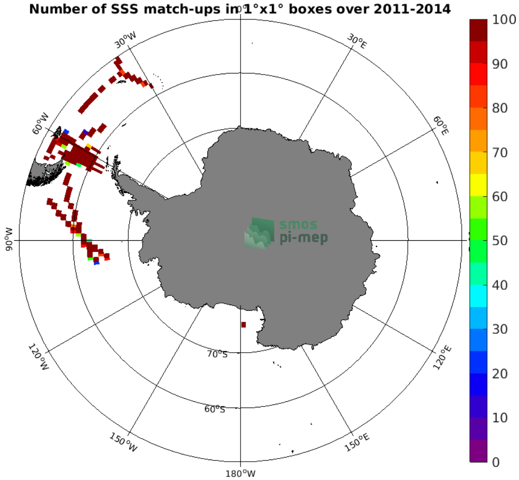
Figure 4: Number of SSS match-ups between TSG (SAMOS) SSS and the Aquarius SSS L3 CAP v5 - 7-Day running (JPL) SSS product for the Southern Ocean Pi-MEP region over 1°x1° boxes and for the full satellite product period.
